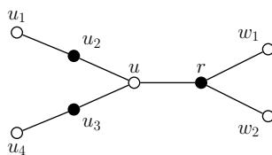
Figure 1: The gadget used in the proof of Theorem 3.5. The white and black vertices are used to denote vertices belonging to different bipartitions.
