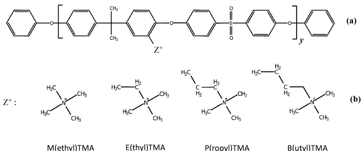
Fig. 1 – Chemical structures of model polymers. (a) PSU; (b): graft ( \text{Z}^+ ) composed of a carbon chain (Methyl, Ethyl, Propyl, Butyl) bonded to an ammonium group (trimethyl ammonium).
