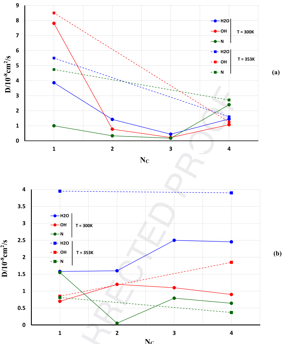
Fig. 4 – Diffusion coefficient of O_w , O_h and N vs. number of carbon atom in the alkyl chain. (a) WU = 10\% ; (b) WU = 20\% . The two values of D_{O_w} ( T = 353 \text{ K} - WU = 20\% ) in figure (b) are divided by 4.
