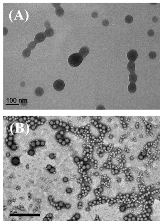
Fig. 4. Electron micrograph of unstained poly(isobutylcyanoacrylate) NPs deposited on a formvar-carbon coated copper grid for EM. (A) Projected image of single particles appeared circular suggesting that the particles were spherical. In contrast, particles included in aggregates appeared distorted due to the close contact with their neighbors. Scale bar: 100 nm. (B) Segregation according to particle size occurred during sample preparation of a highly polydisperse dispersion of the NPs. Scale bare: 2 μm. Evaluation of shape, size and PSD by EM requires that NPs will be well individualized on the sample holder and randomly distributed over the surface of the sample holder.
