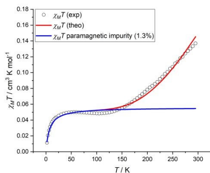
Figure 4 Variable-temperature magnetic susceptibility of solid 1 in the range 2–295 K ( B = 0.5 T). The coupling constant J = -348 \text{ cm}^{-1} was determined using \hat{H} = -2J\hat{S}_A \cdot \hat{S}_B with g_1 = g_2 = 2.0 (fixed).
