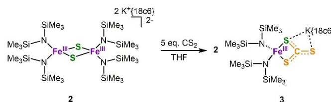
Scheme 2. Reaction of 2 with \text{CS}_2 to the thiocarbonate complex 3 .
