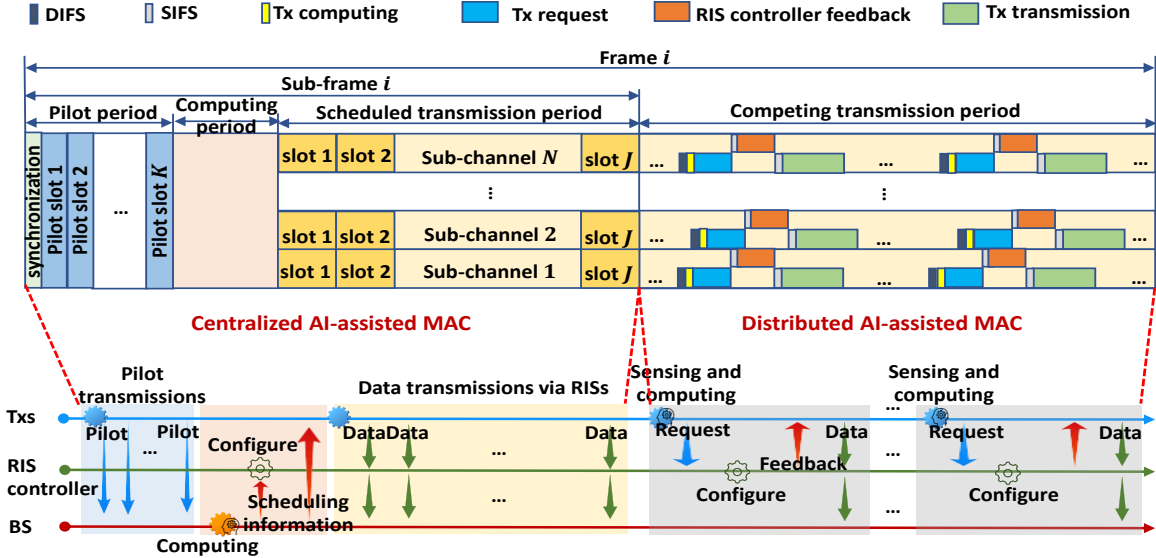
Fig. 3: Hybrid AI-assisted MAC structure with centralized and distributed designs, an illustration of Case 1.
