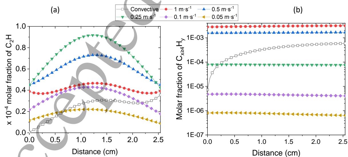
Figure 14: \text{C}_2\text{H} radical (a) and large hydrocarbon (b), i.e., \text{C}_{x \geq 4}\text{H}_y , mole-fraction in the gap for convective (blank square) and MCDS (solid symbol) boundary conditions with different inlet flow velocity-values
