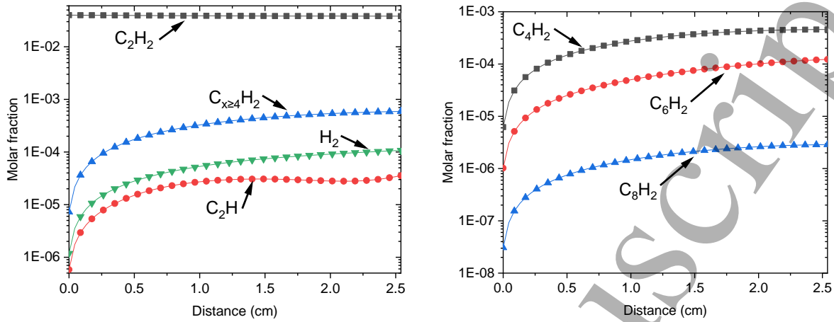
Figure 5 : distribution of (a) \text{H}_2 , \text{C}_2\text{H} , \text{C}_2\text{H}_2 , and large hydrocarbons (lumped for x=4,6,8 ) and (b) \text{C}_4\text{H}_2 , \text{C}_6\text{H}_2 and \text{C}_8\text{H}_2 along the discharge in \text{Ar}/\text{C}_2\text{H}_2 discharge. for convective boundary conditions
