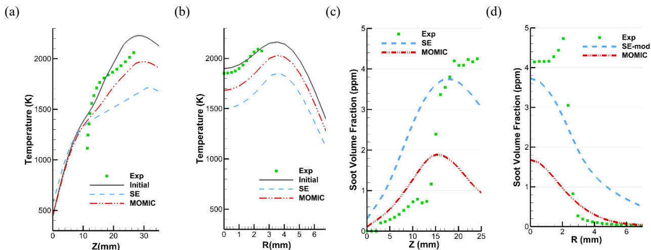
Figure 3. Temperature (left) and soot volumetric fraction (right) profiles along the centerline (a) and (c) and the radial direction (b) and (d). In this figure, Exp, SE and MOMIC correspond to, respectively, experimental data, semi-empirical with radiation, MOMIC with radiation.
