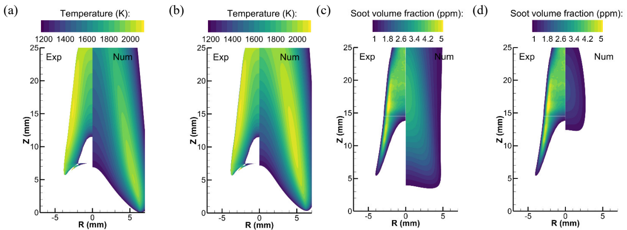
Figure 2. Temperature (left plots) and soot volumetric fraction (right plots) contours for the semi-empirical model [(a) and (c)], and the MOMIC one [(b) and (d)]. Experimental data (Jerez et al., 2019) shown on the left side of each plot.
