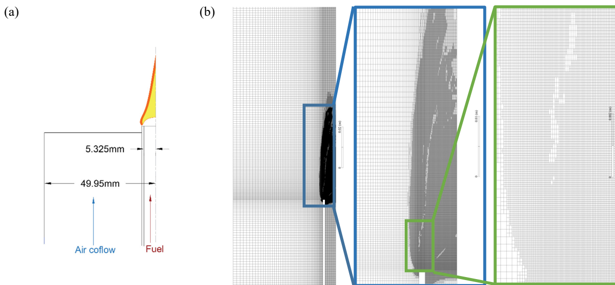
Figure 1. (a) Scheme of Gülder burner. (b) Computational mesh generated in ANSYS Meshing (ANSYS, 2021b) and adapted in ANSYS Fluent (ANSYS, 2021a).
