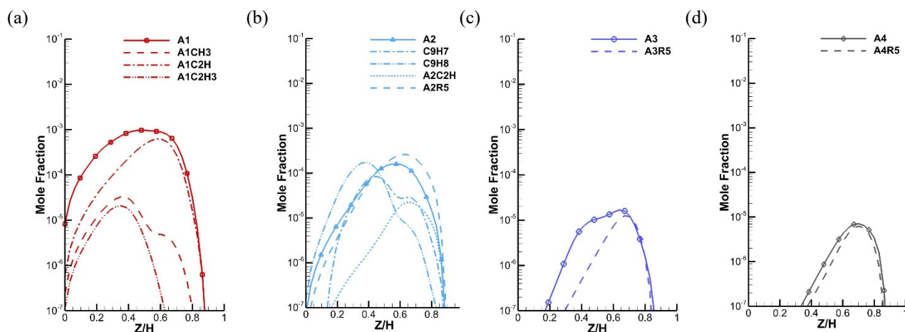
Figure 5. Mole fractions of PAH grouped by (a) one, (b) two, (c) three and (d) four aromatics rings.
