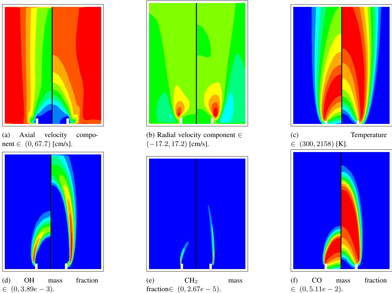
Figure 2: Comparison of the flame structures obtained with CFD for the lower, v_{f,i} = 1.75 cm/s, (left) and higher, v_{f,i} = 4.38 cm/s, (right) prescribed fuel inlet velocity. The color map goes from blue (minimum) to red (maximum).
