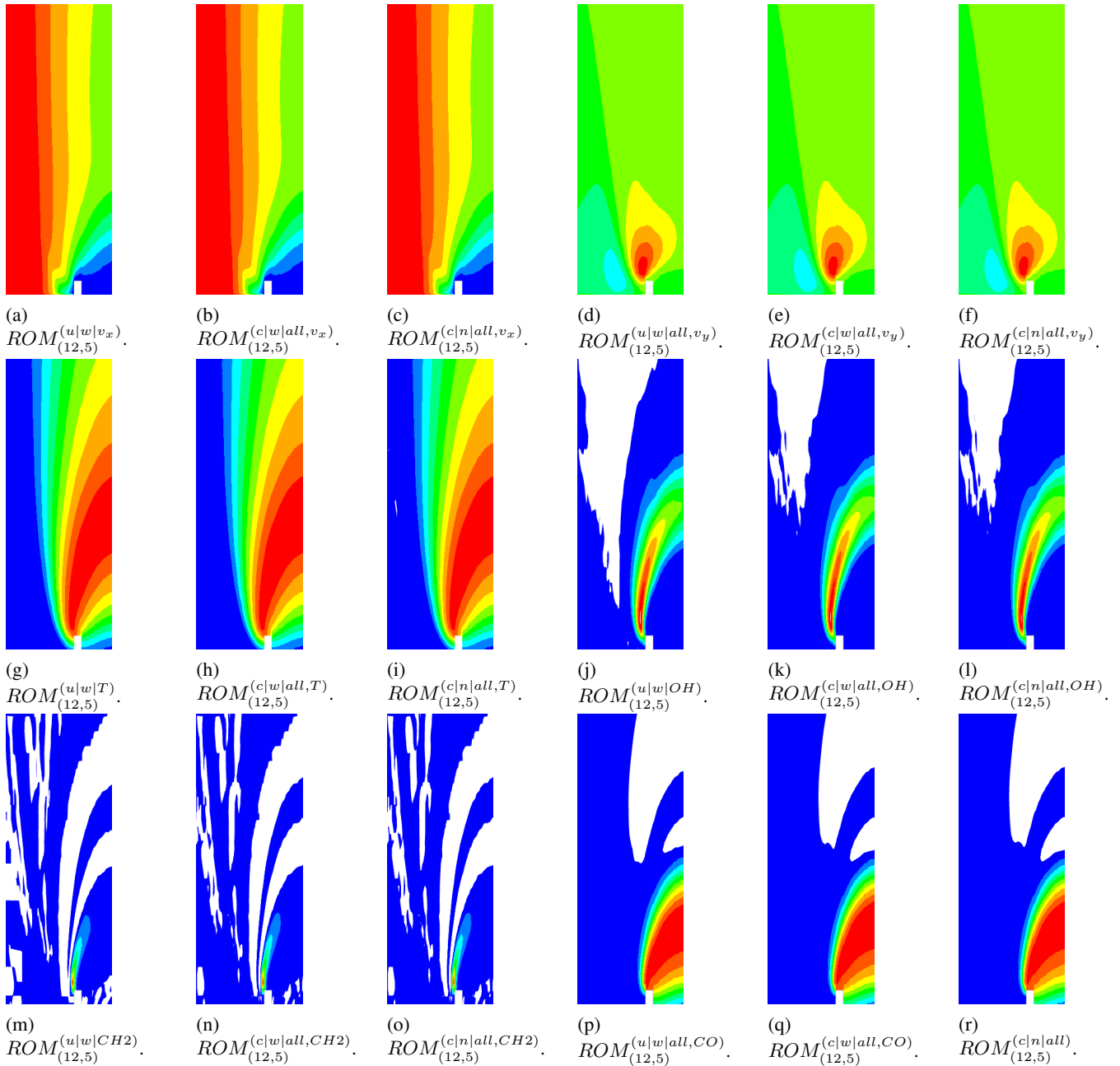
Figure 6: Comparison of the results obtained with reduced order model using 5 modes for the properties treated uncoupled ( ROM_{(12,5)}^{(u|w|p)} ), coupled without normalization ( ROM_{(12,5)}^{(c|w|all)} ) and coupled with the temperature and components of velocity normalized ( ROM_{(12,5)}^{(c|n|all)} ); for the validation case with prescribed fuel inlet velocity of v_{f,i} = 2.11 cm/s. The axial component of the velocity (a,b and c) varies between 0 to 64.6 cm/s; the radial component of velocity (d, e and f) varies (-16, 16) cm/s; the temperature (g, h and i) varies between (300, 2, 141) K. The OH mass fraction (j, k and l) varies between 0 to 3.71 \cdot 10^{-3} ; the CH 2 mass fraction (m, n and o) varies [0, 2.83 \cdot 10^{-5}] ; the CO mass fraction (p, q and r) varies between [0, 5.1 \cdot 10^{-2}] . The color map goes from blue (minimum) to red (maximum). The fuel inlet is located in the bottom right side, and in the left side is the air inlet.
