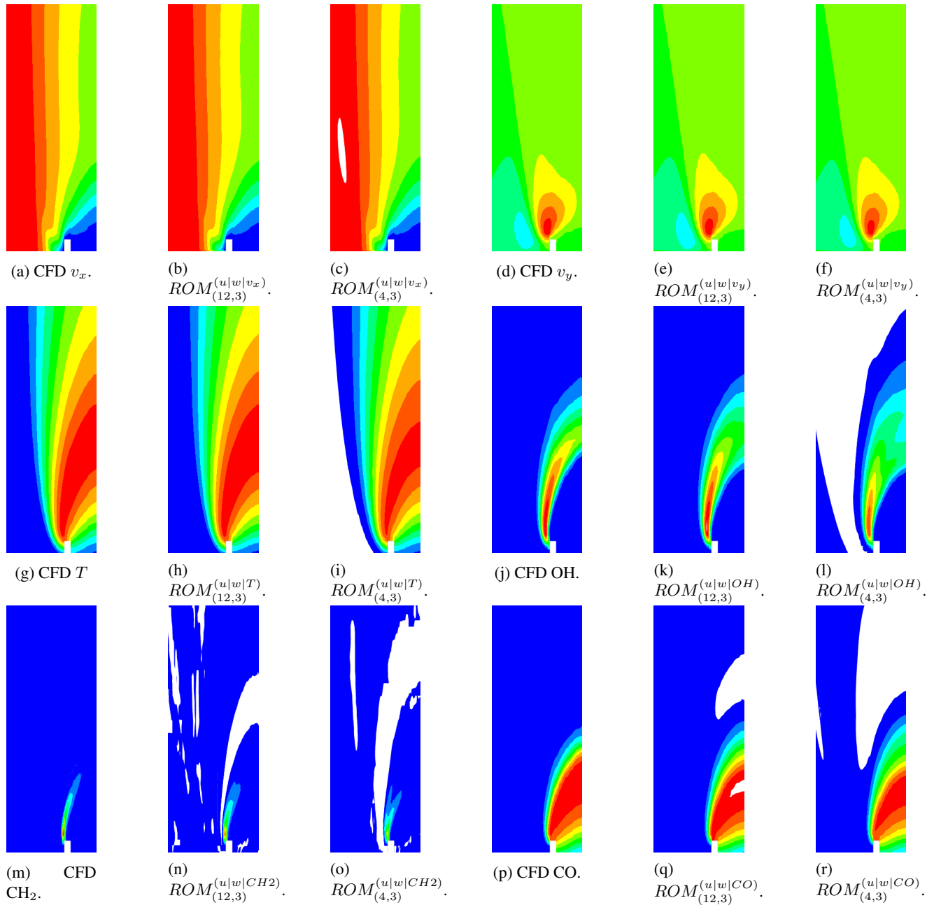
Figure 4: Comparison of the results obtained with computational fluid dynamics (CFD), and reduced order model using 12 learning cases ( ROM_{(12,3)}^{(u|w|p)} ) and 4 learning cases ( ROM_{(4,3)}^{(u|w|p)} ), for the validation case with prescribed fuel inlet velocity of v_{f,i} = 2.11 cm/s. The axial component of the velocity (a,b and c) varies between 0 to 64.6 cm/s; the radial component of velocity (d, e and f) varies (-16, 16) cm/s; the temperature (g, h and i) varies between (300, 2, 141) K. The OH mass fraction (j, k and l) varies between 0 to 3.71 \cdot 10^{-3} ; the CH_2 mass fraction (m, n and o) varies [0, 2.83 \cdot 10^{-5}] ; the CO mass fraction (p, q and r) varies between [0, 5.1 \cdot 10^{-2}] . The color map goes from blue (minimum) to red (maximum). The fuel inlet is located in the bottom right side, and in the left side is the air inlet.
