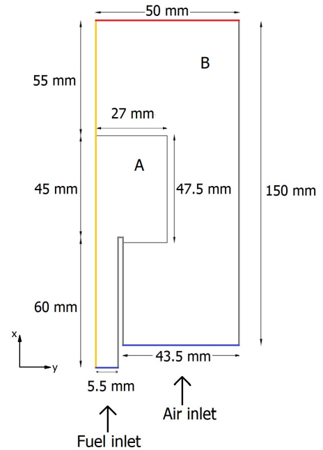
Figure 1: Representation of the Gülder burner domain and its dimensions. (A): internal part, (B): external part.
