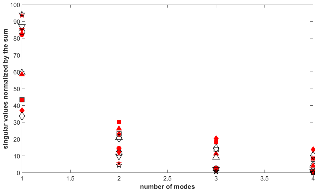
Figure 3: Singular values normalized by the sum \times number of modes. Filled symbols: ROM using 4 learning cases; non-filled symbols: ROM using 12 learning cases. \nabla : temperature; \star : axial velocity component; \circ : radial velocity component; \square : OH mass fraction; \diamond : CH 2 mass fraction; \triangle : CO mass fraction.
