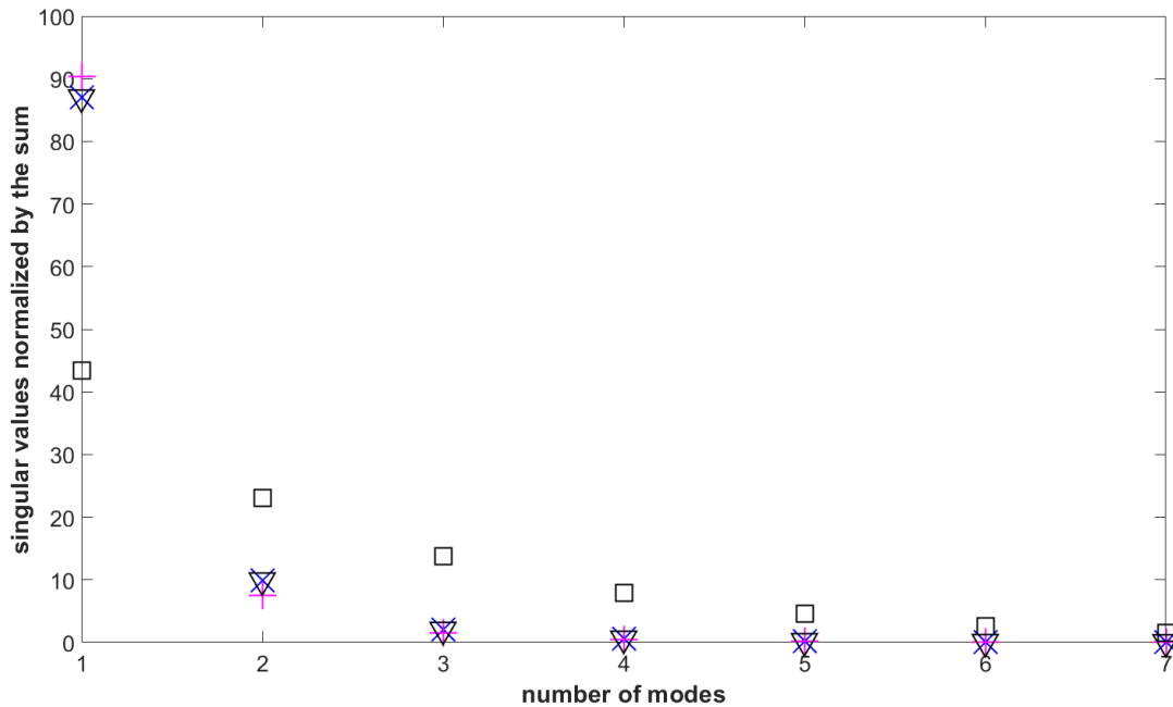
Figure 5: Singular value normalized by the sum \times number of modes. \nabla : temperature; \square : OH mass fraction; \times : Properties treated as coupled, without normalization; + : Properties treated as coupled, with temperature and velocity components normalized.
