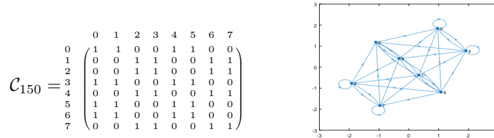
Figure 1: (left) The transition matrix \mathcal{C}_{150} for |\omega| = 3 . (right) Graph of \mathcal{C}_{150} .
