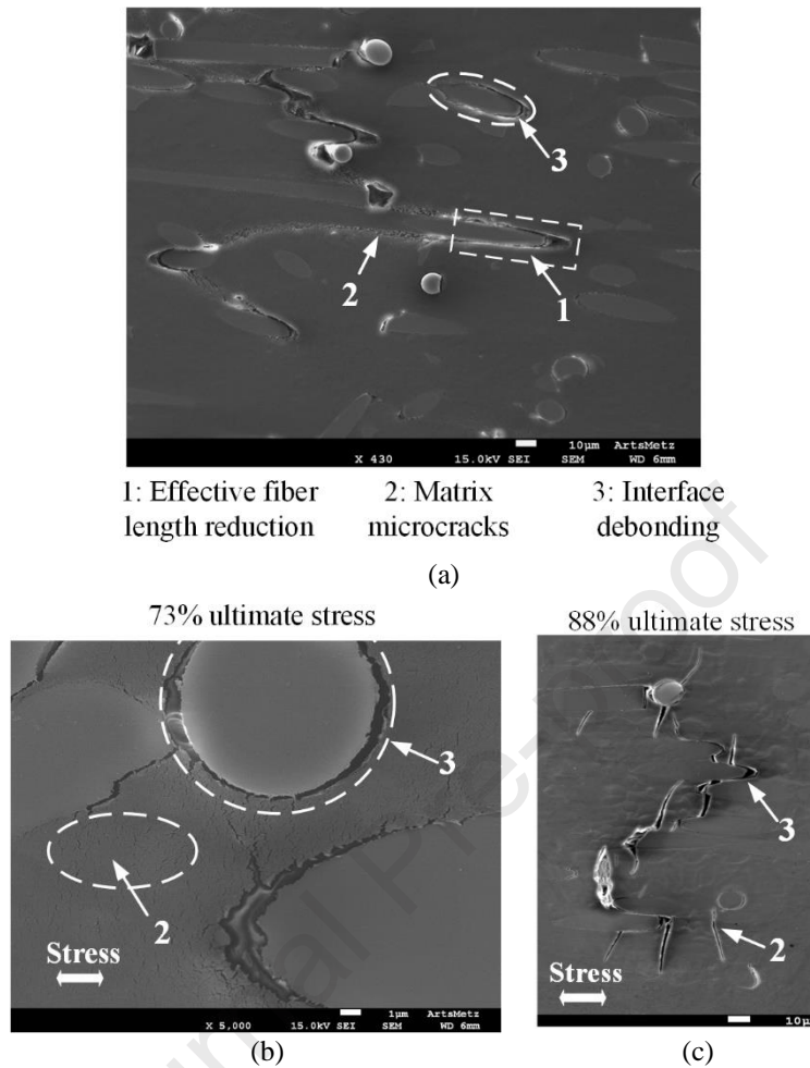
Figure 2 Damage mechanisms in short glass-fiber reinforced polyamide composites (PA66/GF) as reported by Arif et al. (2014a): (a) effective fiber length reduction, matrix microcracks and interface debonding observed experimentally; matrix microcracks and interface debonding at (b) 73% and (c) 88% ultimate stress levels observed via the in-situ SEM 3-point bending test. The observations are carried out in the tension zone (skin-shell region).
