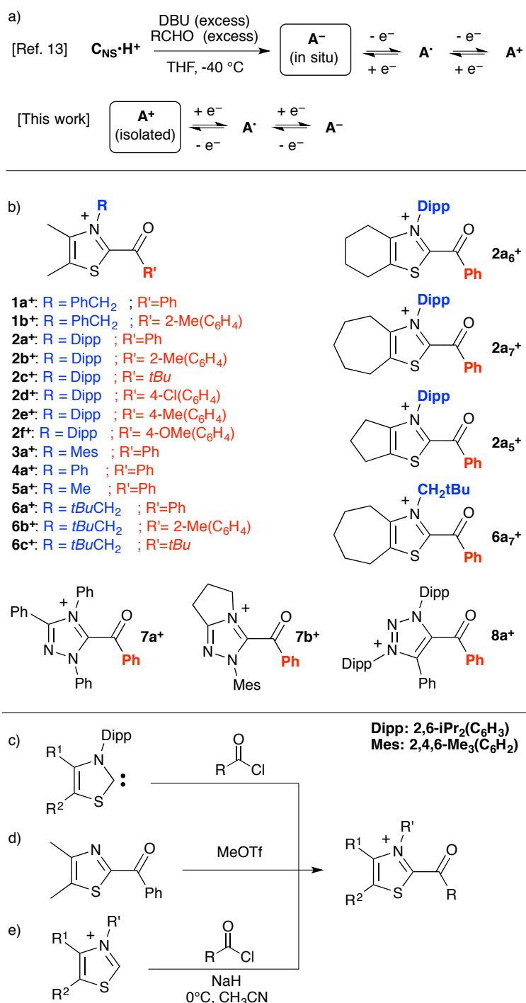
Scheme 1: (a) generation of enolates A - and in situ electrochemical study according to ref. 13; (b) Structure of acylazoliums 1 + -8 + ; synthesis of acyl thiazolium by: (c) acylation of persistent carbenes, (d) alkylation of an acyl thiazole or (e) in situ trapping of transient carbenes with acyl chlorides.
