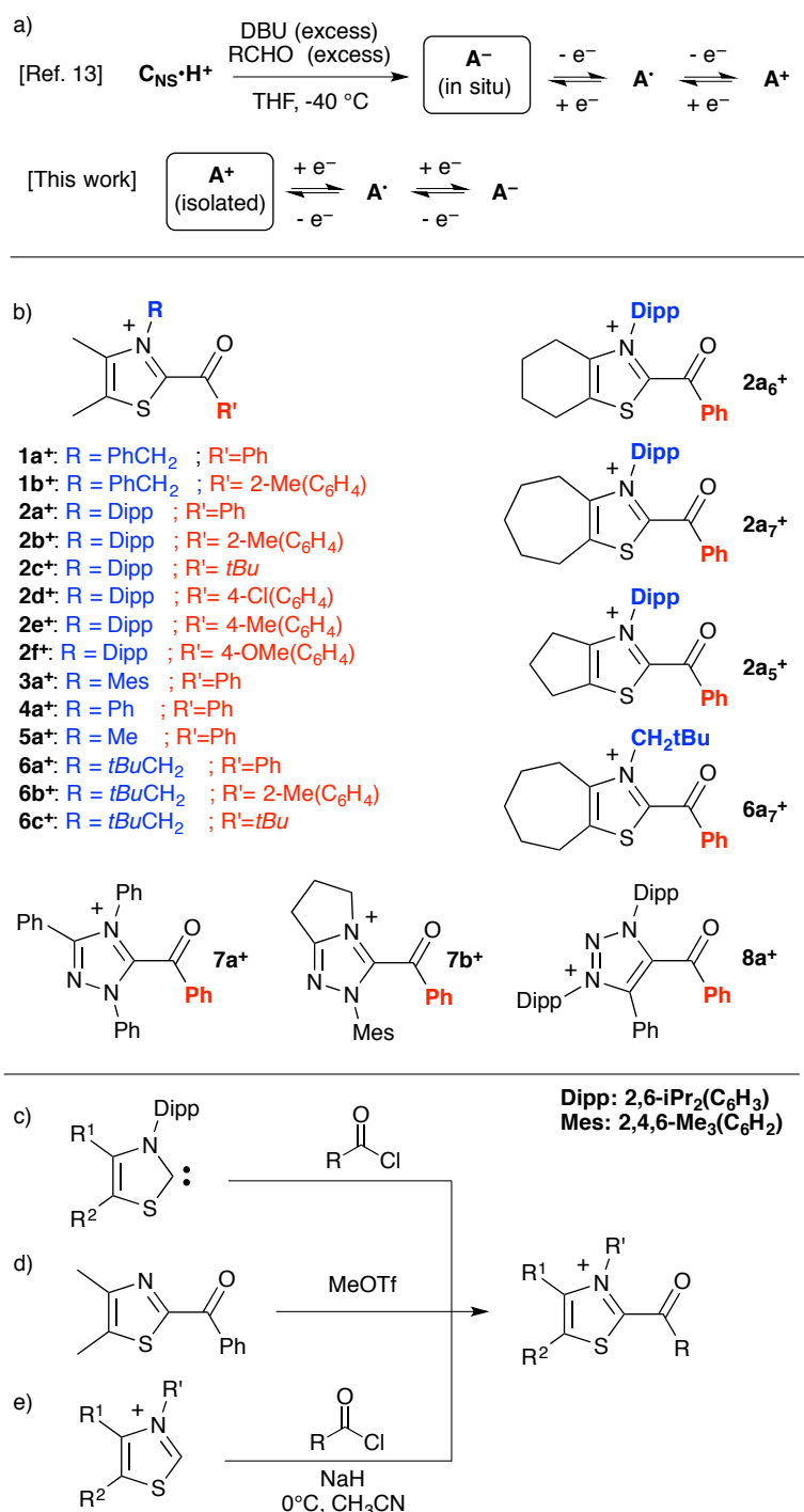
Scheme 1: (a) generation of enolates \text{A}^- and in situ electrochemical study according to ref. 13; (b) Structure of acylazoliums 1 + - 8 + ; synthesis of acyl thiazolium by: (c) acylation of persistent carbenes, (d) alkylation of an acyl thiazole or (e) in situ trapping of transient carbenes with acyl chlorides.
