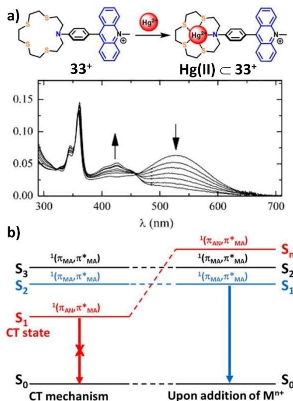
Figure 12. a) UV-Vis spectra of T. del Giacco's receptor (33 + ) upon addition of Hg 2+ ions in water and b) the schematized energy diagram explaining the change in absorption (AN: Aniline, MA: Methylacridinium). Reproduced from reference [42] with permission from Royal Society of Chemistry.
