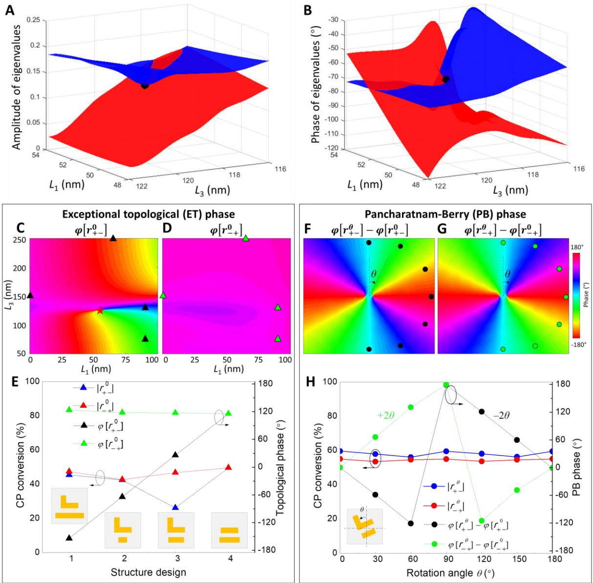
Fig. 3. Simulation results of the metasurface in the parameter space R = (L_1, L_3) . (A) Simulated amplitude and (B) phase of two eigenvalues at \lambda = 600 \text{ nm} . A self-intersecting Riemann surface profile is observed. The EP is highlighted as black dot, where two eigenvalues degenerate at (L_1, L_3) = (52 \text{ nm}, 119 \text{ nm}) . (C) Simulated ET phase of r_{+-}^0 and (D) nearly constant phase of r_{-+}^0 . (E) Four meta-atom designs are selected such that the ET phase interval is 90^\circ , highlighted as triangles in C and D. The inset figures are four corresponding structure designs. (F) Simulated PB phase of r_{+-}^\theta and (G) r_{-+}^\theta , where the presented phase has been subtracted by the original phase of r_{\pm\mp}^0 without rotation to display PB phase only. (H) Seven rotated structures are presented with rotation angle from 0^\circ to 180^\circ stepped by 30^\circ , highlighted as dots in F and G. (See more details in Supplementary fig. S11 and S14).
