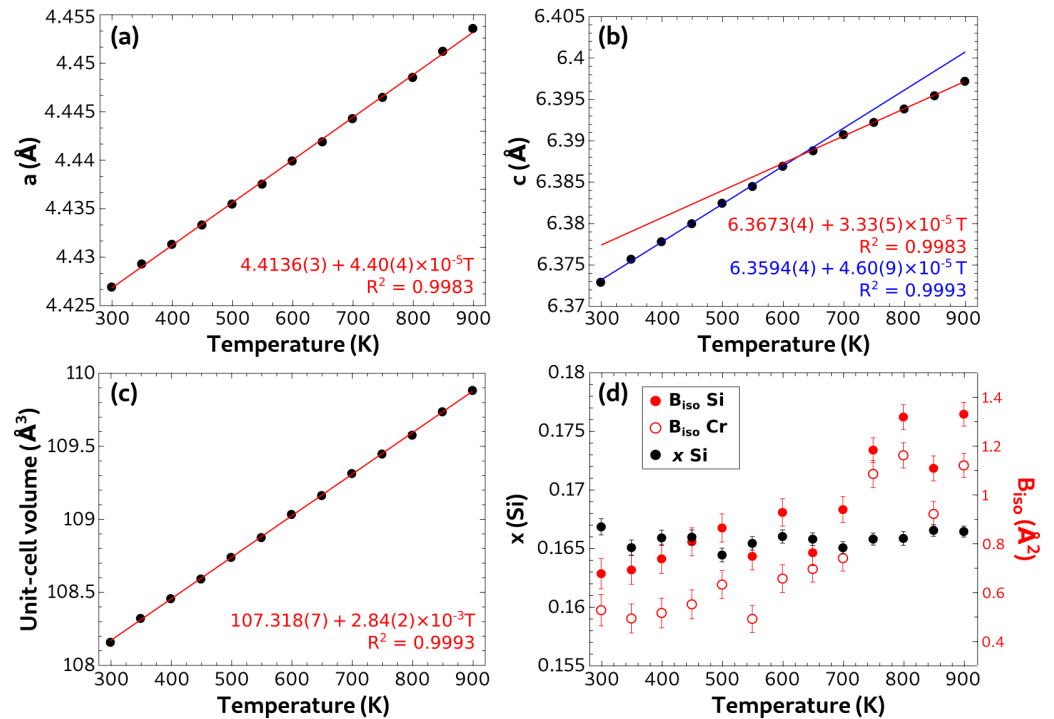
Figure 3. Thermal evolution of the lattice parameters (a) a and (b) c , (c) the unit cell volume and (d) the positional parameter x in black and the global isotropic atomic displacement parameters B_{iso} in red.
