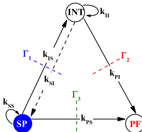
Figure 6. Markov diagram for the three-state system that models the unimolecular dissociation in the gas phase.
