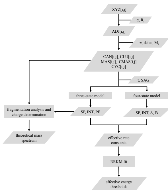
Figure 11. Schematic flowchart summarizing the present approach. We report the different matrices obtained in their sequence and the different parameters, states and properties as defined in the text.
