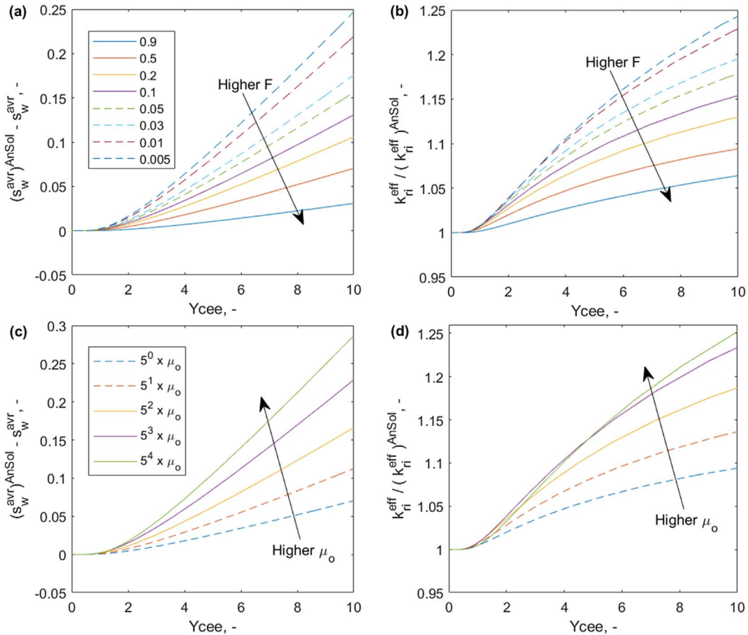
Fig. 10. The difference between general solutions and the analytical solution in terms of (\bar{s}_w)^{\text{AnSol}} - \bar{s}_w in (a) and (c) and \frac{k_{ri}^{\text{eff}}}{k_{ri}^{\text{AnSol}}} in (b) and (d) for changes in flow fraction F in (a) and (b) and changes in oil viscosity in (c) and (d). All results are plotted against Y_{\text{cee}} and demonstrate that the analytical solution is valid for Y_{\text{cee}} < 1 .
