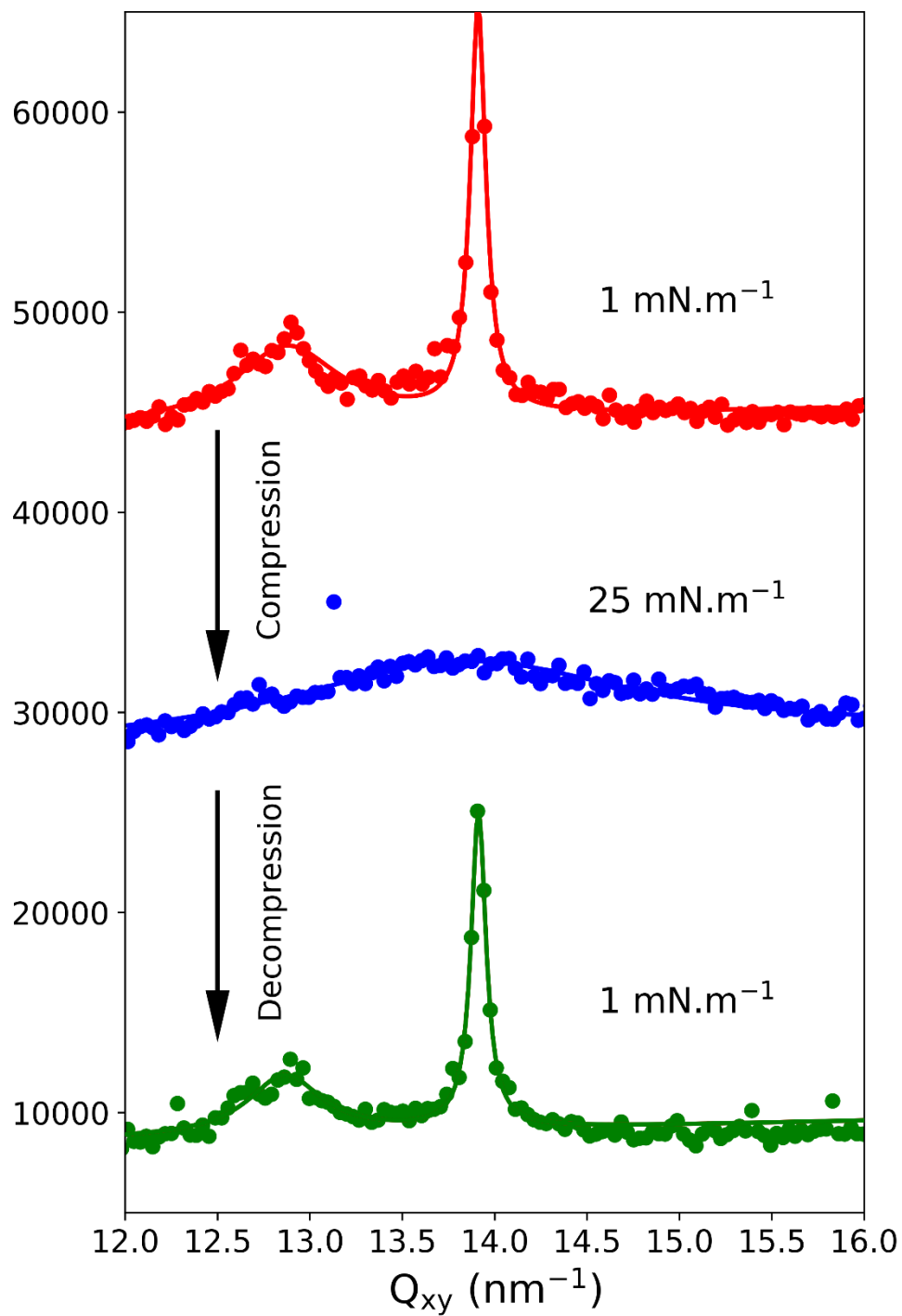
Figure 6. Q_z integrated GIXD spectra of 13-4OH monolayer at 12°C: up to bottom: \pi = 1 \text{ mNm}^{-1} in compression, \pi = 25 \text{ mNm}^{-1} and \pi = 1 \text{ mNm}^{-1} in decompression.
