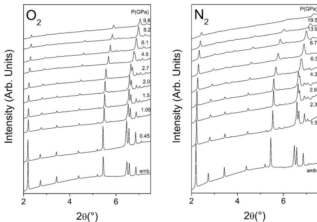
Figure 3. X-ray diffraction patterns of TON in O_2 and N_2 as a function of pressure ( \lambda=0.41121 \text{ \AA} ). The diffraction lines of \epsilon - O_2 and \epsilon - N_2 were observed above 10 GPa at diffraction angles above 8^\circ . They exhibited strong texture and were typically more than an order of magnitude higher in intensity than the diffraction lines of TON indicating that the latter was completely immersed in a large amount of bulk O_2 or N_2 pressure transmitting medium
