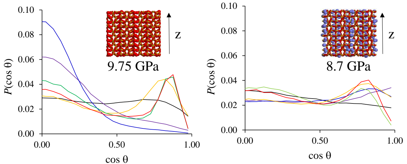
Figure 9. Simulated angular distributions P(\cos \theta) for \text{O}_2 (left) and \text{N}_2 (right) confined in TON at room temperature and different pressure. \theta is the angle between the molecule axis and the z-axis which corresponds to the channel axis in TON. For \text{O}_2 , the color code is P = 1.05 GPa (black), 1.95 GPa (purple), 3.5 GPa (blue), 5.09 GPa (orange), 8.17 GPa (green), and 9.75 GPa (red). For \text{N}_2 , the color code is 1.5 GPa (black), 2.25 GPa (purple), 2.6 GPa (blue), 4.3 GPa (orange), 6.3 GPa (green), and 8.7 GPa (red). For each gas, we also show a typical molecular configuration with the same color code as in Fig. 5 (the red and blue spheres are the O and N atoms in \text{O}_2 and \text{N}_2 , respectively).
