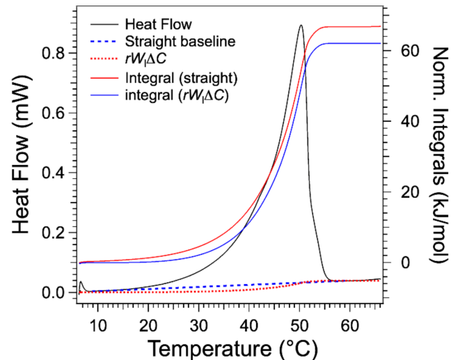
Figure 6. Thermogram of HSA/nitrobenzene (0.03 wt. fraction). Integration of the heat flow after subtraction of two different baselines. The straight baseline is the one subtracted from the commercial software. The other baseline is rW_1\Delta C_p ( W_1 calculated from Equation (8) and normalized to match the value of the plateau after the transition \approx W\Delta C_p and multiplied by the heating rate r to convert the quantity to heat flow).
