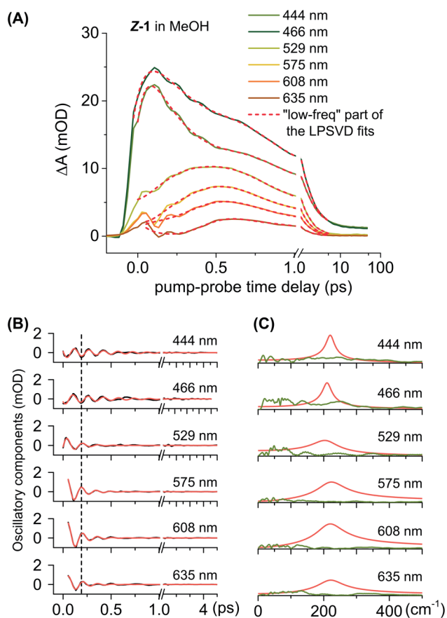
Fig. 5 LPSVD analysis of the Vis ESA kinetic traces of Z_S -1 in methanol, evidencing signatures of vibrational coherent motion in S_1 . (A) Selection of TA kinetic traces recorded in the high-energy side ( <500 \text{ nm} ) and low-energy side ( >500 \text{ nm} ) of the Vis ESA band. The red dotted lines are reconstructed including only the low-frequency components – i.e. <100 \text{ cm}^{-1} – of the LPSVD fit of the kinetics traces. (B) The oscillatory part of the TA signal (black lines, computed as the difference between the TA kinetics and the red dotted curves in panel A) are compared with the high-frequency part ( >100 \text{ cm}^{-1} only, red curves) of the LPSVD fit. (C) LPSVD spectrum (red) of the red traces in panel B, compared with the Fourier transform (FFT, green) of the residuals of the LPSVD fit. The spectral amplitude associated with the prominent vibrational mode at \sim 215 \text{ cm}^{-1} is about 3 to 10 times larger than the average spectral amplitude of the fit residuals.
