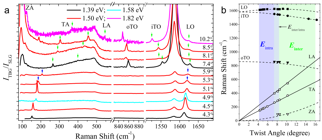
Figure 1. (a) Raman spectra of ten TBG samples with different angles between 4.3^\circ and 10.2^\circ . The spectra were acquired using four different laser lines, represented by different colours in the figure, but only those presenting the strongest resonance effect are displayed in the figure. The spectra is shown in three regions: (i) the acoustic modes (ZA, TA and LA), (ii) the out-of-plane TO phonon (oTO) and (iii) the optical modes close to the G band (iTO and LO). All spectra with \theta \geq 7.4^\circ were multiplied by 10 \times in the acoustic and the oTO regions for a better visualisation. (b) Positions of all peaks extracted from all Raman spectra plotted as a function of \theta . The twisting angles were determined by the LA and TA phonon branches according to dispersion curves (full black lines) obtained by Cong et al. 29 (see text). The dashed black lines are theoretical curves of the TBG phonon frequencies 27 as a function of the twisting angle 28 . The blue (green) stripe highlights the range of angles of the TBGs investigated in this work that are activated by the intralayer (interlayer) el-ph process.
