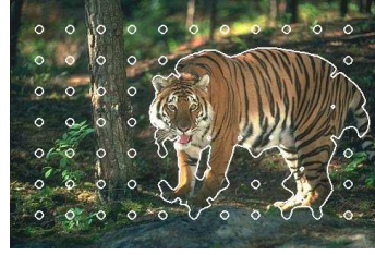
(b) Iteration 200
