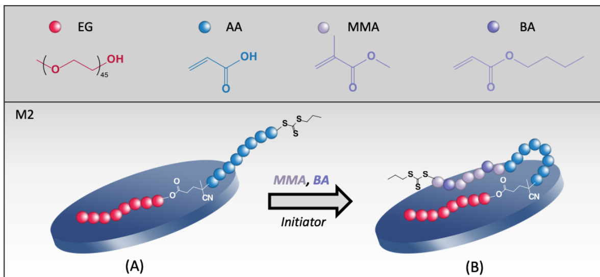
Figure 1 – Schematic representation of Laponite platelets (A) with adsorbed macroRAFT agent PEG 45 - b -PAA 42 -TTC (M2) and (B) during the synthesis of P(MMA- co -BA)/Laponite nanocomposite latexes by RAFT-mediated surfactant-free emulsion polymerization using M2.
