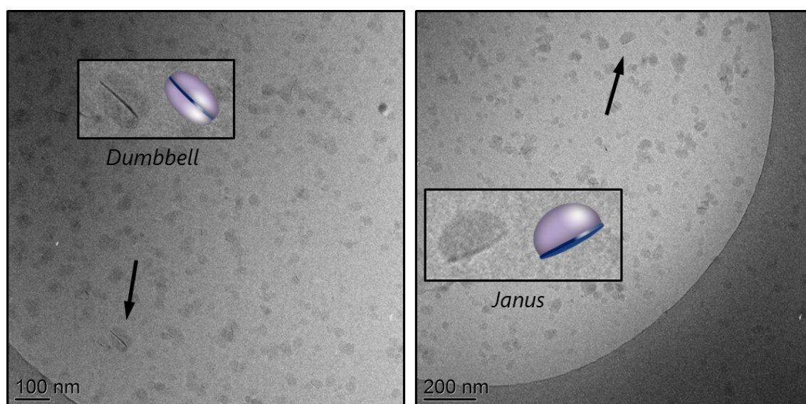
Figure 5. Cryo-TEM images of hybrid particles obtained by the copolymerization of MMA:BA 90:10, at 80 °C, in the presence of 2.2 mM of macroRAFT agent P(AA 16-co -BA 16 )-TTC (M6) and 5 g L -1 of Laponite at pH 7.5 (R6).
