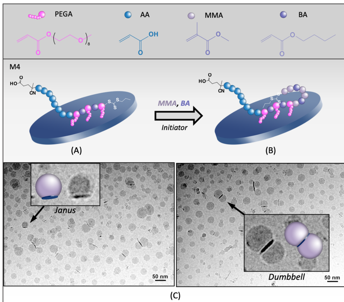
Figure 3 – Schematic representation of Laponite platelets (A) with adsorbed macroRAFT agent PAA 40 - b -P(PEGA 6 - co -BA 4 )-TTC (M4) and (B) during the synthesis of P(MMA- co -BA)/Laponite nanocomposite latex by RAFT-mediated surfactant-free emulsion polymerization using M4. (C) Cryo-TEM images of hybrid particles obtained by the copolymerization of MMA:BA 80:20, at 80 °C, in the presence of 2.2 mM of M4 and 5 g L -1 of Laponite at pH 7.5 (R4B).
