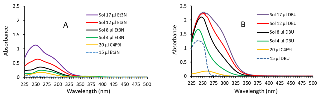
Figure 1: UV-Vis absorption spectra of solutions of C_4F_9I (20 \mu l) in CH_3CN (1 ml) containing increasing amounts of Et_3N (A) or DBU (B) (Transmission cell, pathlength 75 \mu m).
