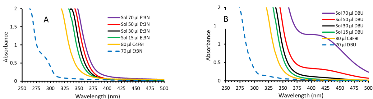
Figure 3: UV-Vis absorption spectra of solutions of C_4F_9I (80 \mu l, 0.46 M) in CH_3CN (1 ml) containing increasing amounts of Et_3N (A) or DBU (B). (Quartz cuvette, pathlength 10 mm). The spectra of C_4F_9I , Et_3N and DBU in CH_3CN (1 ml) are reported for comparison.
