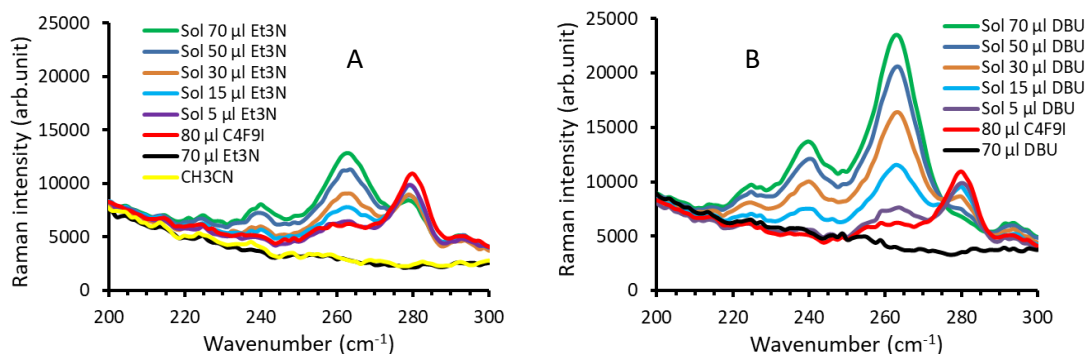
Figure 5: Raman spectra of solutions of C_4F_9I (80 \mu l , 0.46 M) in CH_3CN (1 ml) containing increasing amounts of Et_3N (A) or DBU (B) (Quartz cuvette, pathlength 10 mm). The spectra of C_4F_9I , Et_3N and DBU in CH_3CN (1 ml) are reported for comparison.
