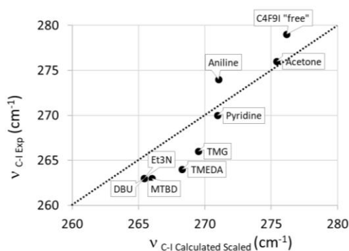
Figure 10: Comparison of the experimental and scaled calculated frequencies at the M06-2X/DGDZVP computational level of the C–I stretching normal mode of “free” C 4 F 9 I and [C 4 F 9 I-LB] complexes. A scaling factor of 0.95 was used to scale the calculated frequencies.[32]
