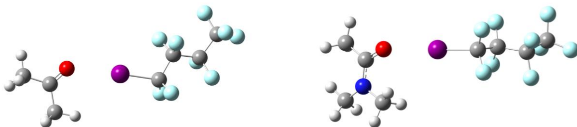
Figure 8: Optimized structure of the [C_4F_9I\text{-acetone}] and [C_4F_9I\text{-DMA}] complexes at the M06-2X level using the DGDZVP basis set.
