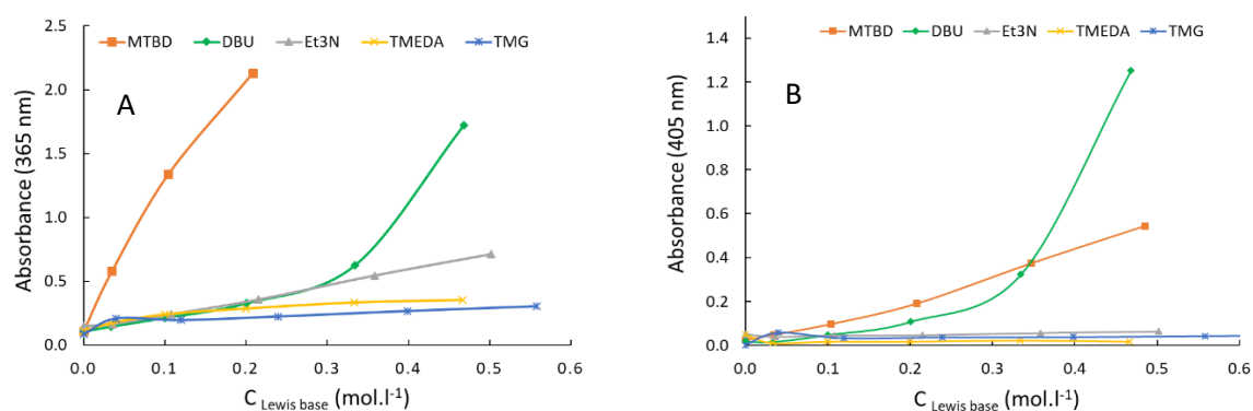
Figure 4: Evolution of the absorbance at 365 nm (A) and 405 nm (B) of CH 3 CN solutions (1 ml) containing C 4 F 9 I (0.46 M) and a Lewis base in as a function of the Lewis base concentration (quartz cuvette, pathlength 10 mm).
