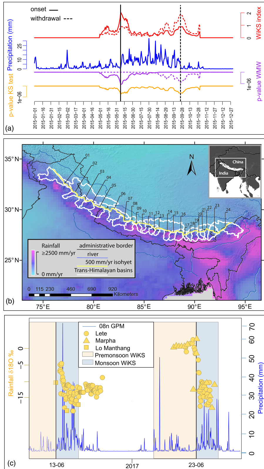
Figure 1. (a) One-year time series of daily precipitation, p values of Kolmogorov-Smirnoff and Wilcoxon-Mann-Whitney tests, and the normalized sum of these two tests (WiKS). Black lines show monsoon boundaries, picked at the WiKS maxima. (b) Map of mean annual precipitation with outlines of 24 Trans-Himalayan Catchments (see names in Table S1). (c) Time series of daily GPM precipitation and rainfall \delta^{18}O in the upper Kali Gandaki valley (08n).
