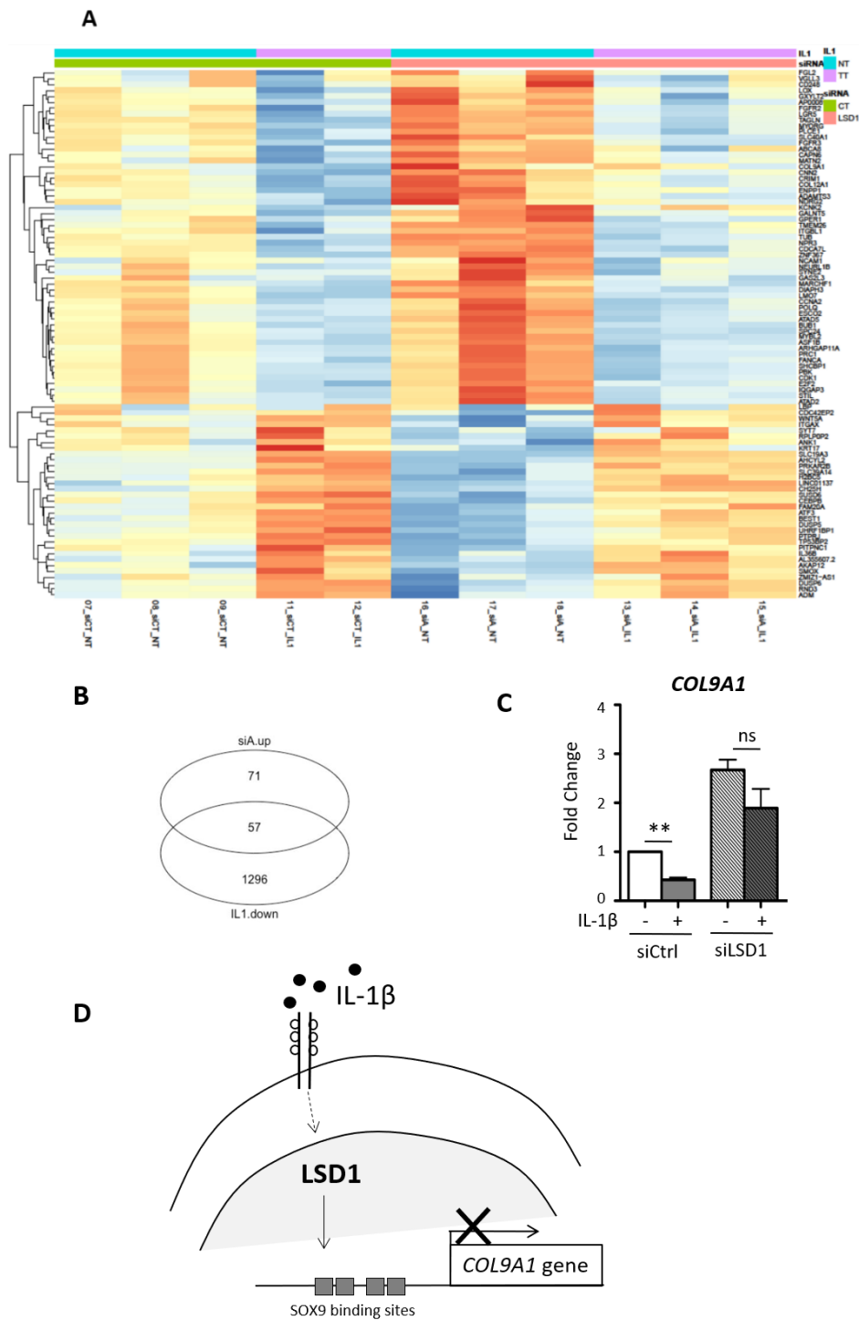
Figure 5. COL9A1 mRNA levels in LSD1-depleted chondrocytes in response to the proinflammatory cytokine IL-1β. Knock-down of LSD1 was realized following human chondrocyte transfection with siRNA and then treated with IL-1β for 24 h. (A) Heatmap of the genes oppositely regulated by LSD1 and IL-1β in articular chondrocytes (NT: non-treated, TT: treated with IL-1β; CT: transfected with siControl, LSD1: transfected with siRNA against LSD1). (B) Diagram indicates 57 genes are simultaneously down-regulated by IL-1β and up-regulated following LSD1 depletion. (C) Real-time PCR was performed from at least 3 independent experiments of additional donors. Results are presented as relative mRNA levels of COL9A1 normalized to RPLP0 ( n = 4 , Student's t -test * p < 0.05 ** p < 0.01 ). (D) Schematic representation showing the down-regulation of COL9A1 by IL-1β is mediated by LSD1.
