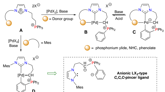
Scheme 1. Preparation of C,C,C-Pincer Pd(II) Complexes featuring NHC and Phosphonium Ylide Cores from N-Phosphonio-Substituted Imidazolium Salts
