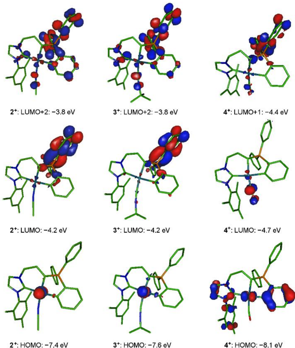
Figure 2. Selected frontier molecular orbitals (energies in eV) of Pd(II) pincer complexes 2^+ (L = NCMc, left ), 3^+ (L = CNtBu, middle ) and 4^+ (L = CO, right ). PBE-D3/6-31G**/LANL2DZ*(Pd) level of calculation.
