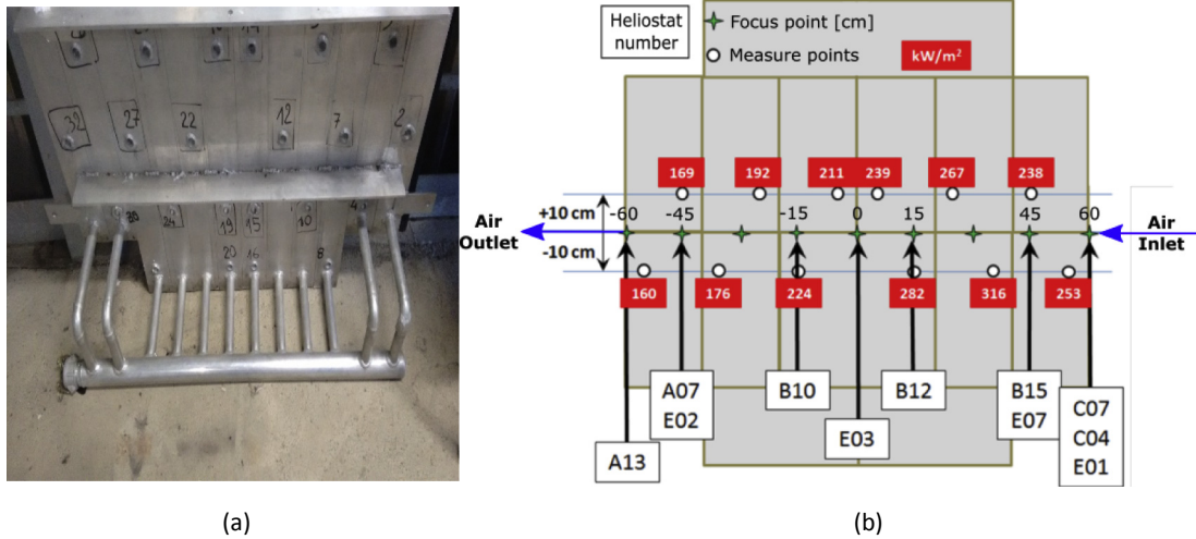
Fig. 13. (a) Image of the dismantled cooled panel (b) Schematic of the cooled panel including the focus point of the 11 heliostats (white rectangles and green crosses) and the intensity of each of the 12 solar flux (red rectangles and white points) for the 07/01/2015 at 16:11 h (civil time).
