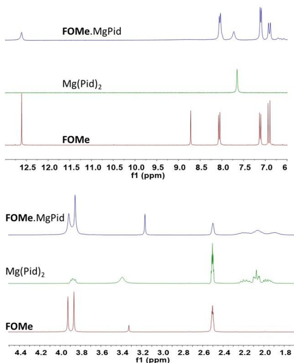
Figure 6. ^1\text{H} NMR spectra of FOMe compared to its isolated magnesium ternary complex FOMe.MgPid and the commercially available \text{Mg}(\text{Pid})_2 . Solvent: \text{DMSO}-d_6
