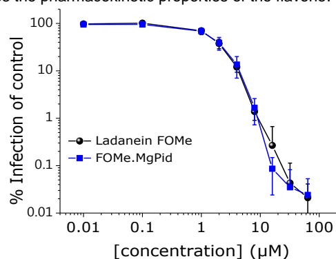
Figure 7. Anti-HCV activities of ladanein and its magnesium pidolate complex. Summary of four independent experiments. HCV Jc-R2a reporter virus was pre-incubated (20 min to 1h) with indicated concentration of drugs at 37 °C prior to infection of Huh-7.5 cells. Cells were subsequently lysed 72 h post infection and luciferase activity was then measured.
