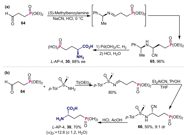
Scheme 20. Strecker reaction for the asymmetric synthesis of L-AP-4.
