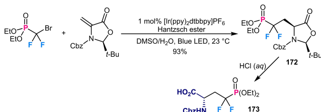
Scheme 64. Chiral auxiliary-induced asymmetric synthesis of the CF 2 -pSer surrogate.
