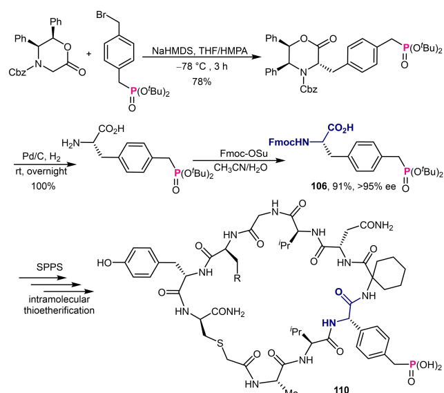
Scheme 40. Chiral diphenyloxazinone-induced asymmetric synthesis of Pmp and cyclotide.
