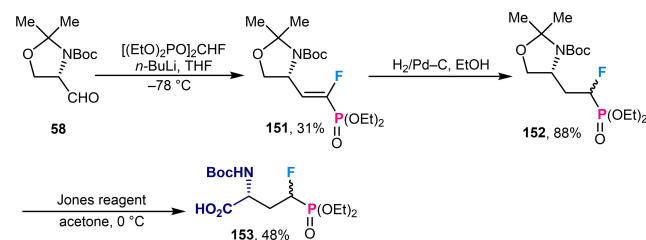
Scheme 56. Chiral Garner's aldehyde-induced asymmetric synthesis of monofluorophosphonomethyl-( R )-serine derivative.
