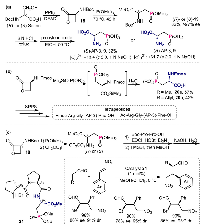
Scheme 7. Asymmetric ring-opening reactions of chiral \alpha -amino- \beta -lactones for the synthesis of 3-phosphonoalanines.
