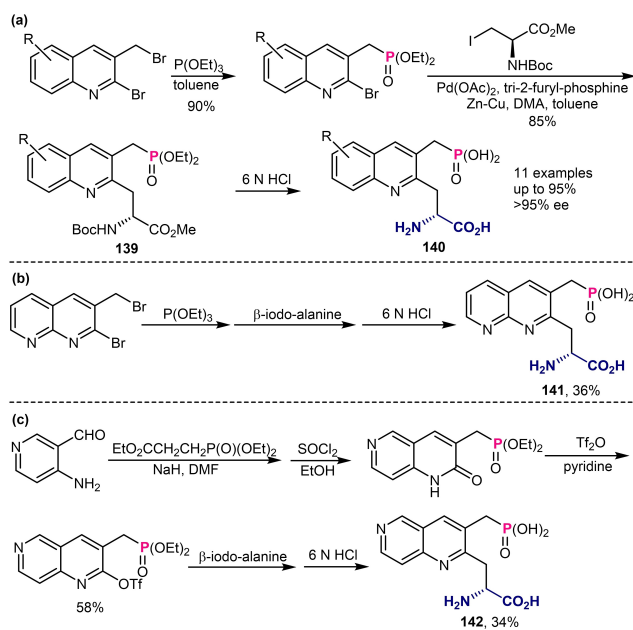
Scheme 52. Asymmetric synthesis of chiral quinolone- and naphthyridine-based phosphono- \alpha -amino acids.
