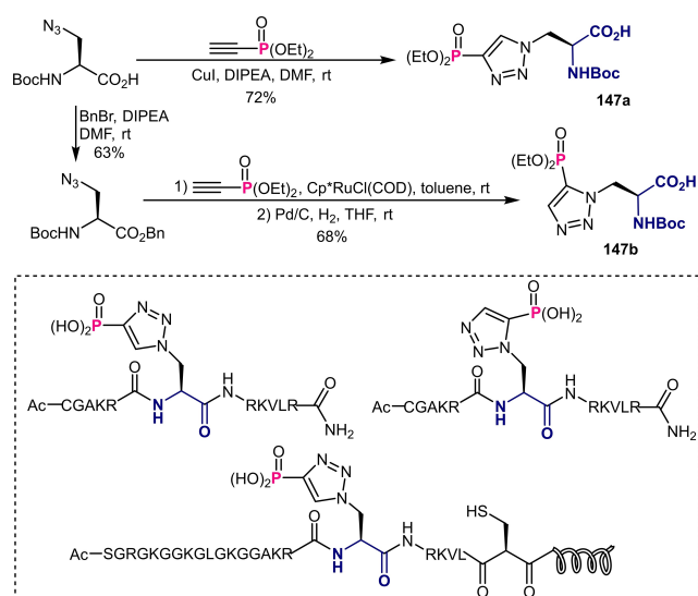
Scheme 54. Asymmetric synthesis of chiral triazole-based phosphono- \alpha -amino acid and the corresponding peptides.
