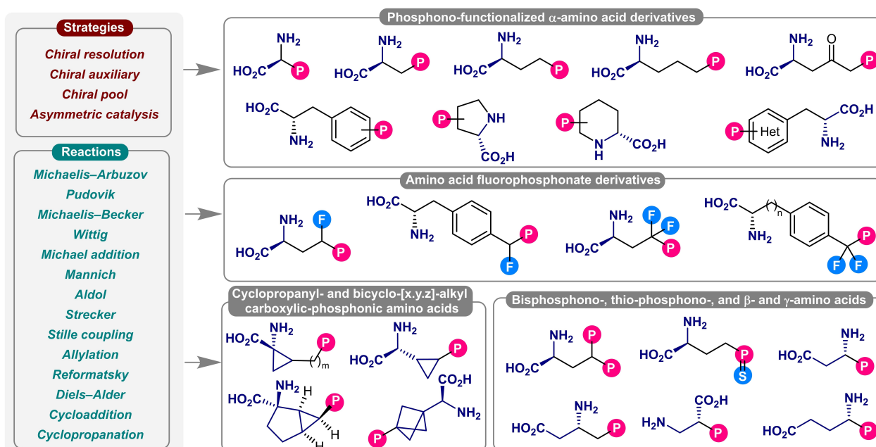
Figure 2. Representative chiral amino carboxylic-phosphonic acid derivatives, key strategies, and reactions.
