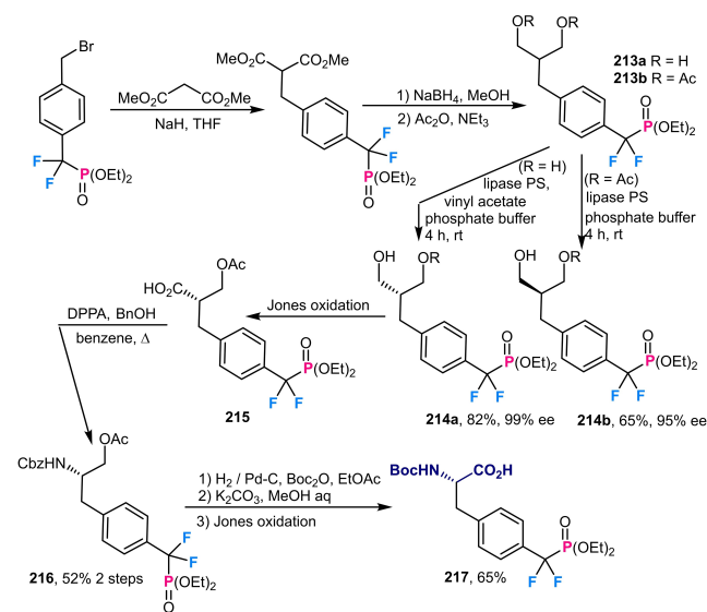
Scheme 78. Enzymatic desymmetrization for enantioselective synthesis of N -Boc-protected L-F 2 Pmp.
