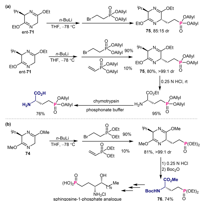
Scheme 24. Asymmetric addition of Schöllkopf bis-lactim ethers for the construction of \gamma -phosphono- \alpha -amino acid derivatives.
