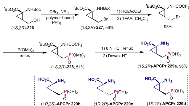
Scheme 82. Asymmetric transformation of chiral cyclopropyl \alpha -amino acids into enantiopure APCPrs.
