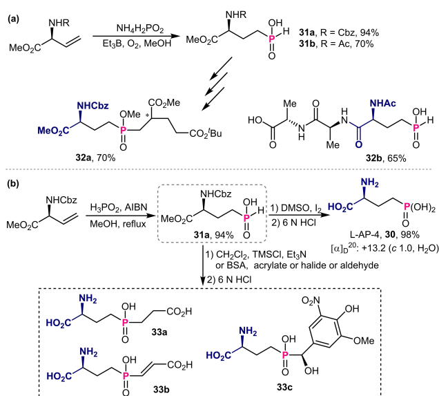
Scheme 12. Asymmetric transformation of vinylglycines into phosphinothricin derivatives.
