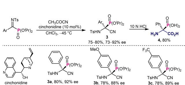
Scheme 2. Catalytic asymmetric Strecker reaction of \alpha -ketimino-phosphonates.
