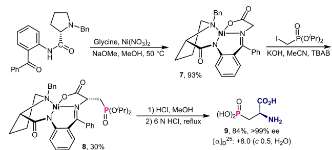
Scheme 4. Asymmetric alkylation of chiral nickel(II) complex 7 for the synthesis of 3-phosphonoalanine.
