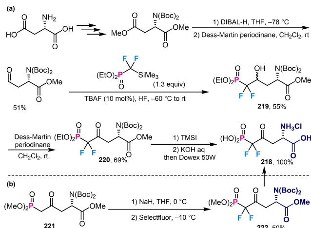
Scheme 79. Asymmetric transformation of aspartic acid into difluorophosphonomethyl aspartic acid analogues.
