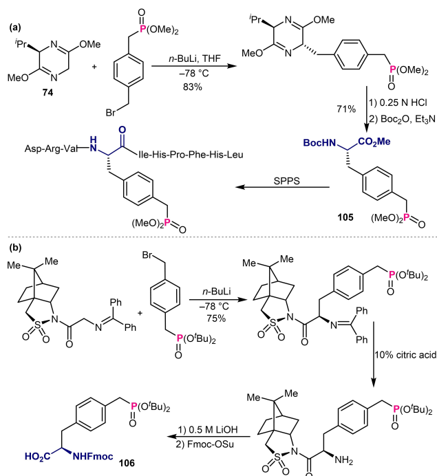
Scheme 38. Schöllkopf bis-lactim ether and camphor sultam imine-induced asymmetric synthesis of Pmps.
