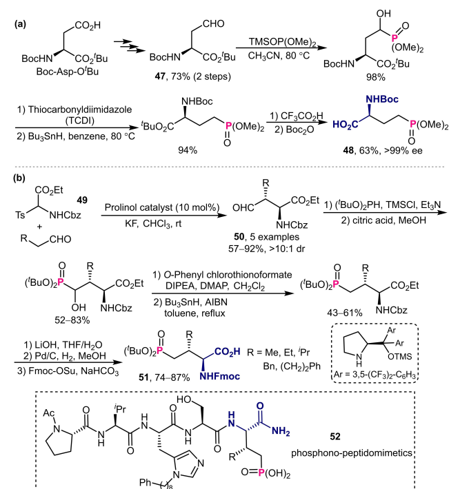
Scheme 15. The Pudovik reaction for the asymmetric synthesis of \gamma -phosphono- \alpha -amino acid derivatives.
