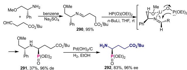
Scheme 98. Catalytic asymmetric synthesis of a chiral \gamma -phosphono- \gamma -amino acid.
