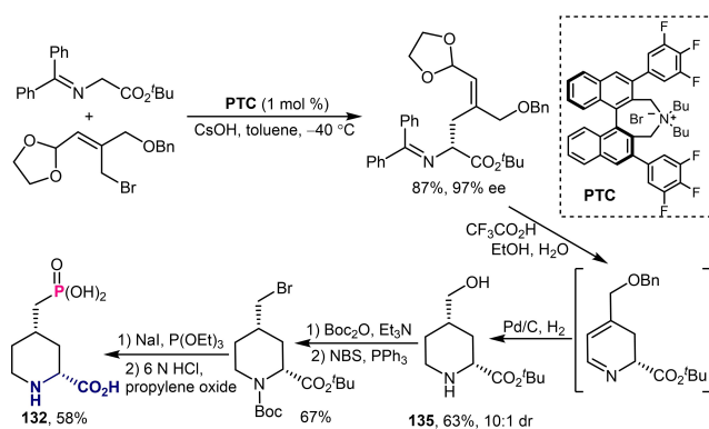
Scheme 50. Catalytic asymmetric synthesis of selfotel.
