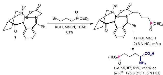
Scheme 30. Asymmetric transformation of chiral Schiff base Ni-complex into \delta -phosphono- \alpha -amino acid L-AP-5.
