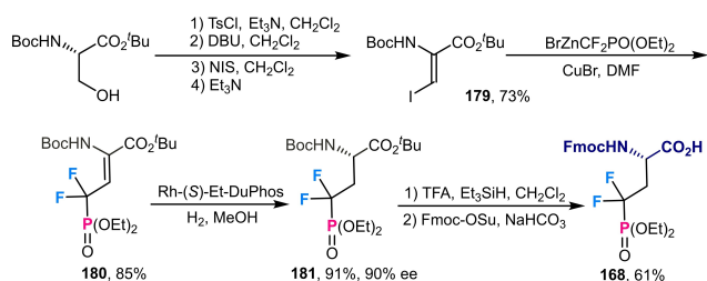
Scheme 67. Catalytic asymmetric hydrogenation for the construction of N -Fmoc-protected CF 2 -pSer.
