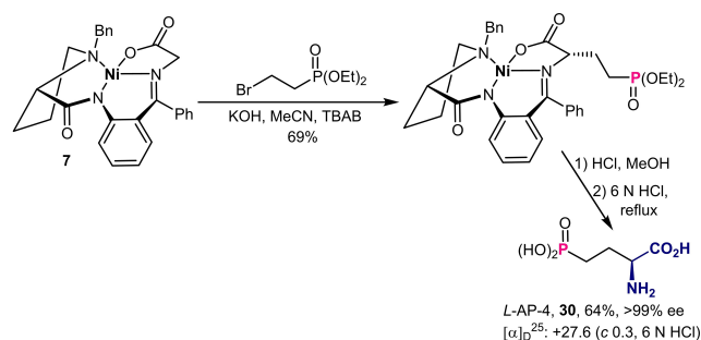
Scheme 21. Asymmetric alkylation of chiral nickel(II) complex 7 for the synthesis L-AP-4.
