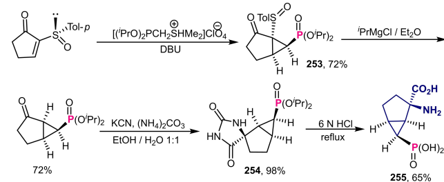
Scheme 88. Asymmetric synthesis of chiral (+)-2-amino-6-phosphono-bicyclo-[3.0.1]-hexane-2-carboxylic acid.
