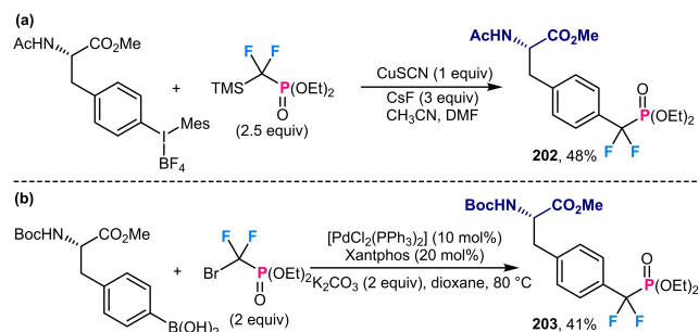
Scheme 74. The cross-coupling of 4-substituted phenylalanines and (EtO) 2 POCF 2 TMS/Br for the asymmetric synthesis of F 2 Pmps.
