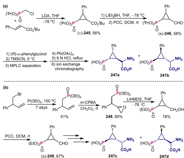
Scheme 86. Chiral auxiliary-induced asymmetric construction of phosphono-phenylcyclopropyl glycine (PPCG) derivatives.
