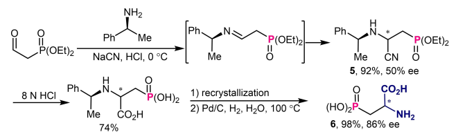
Scheme 3. Asymmetric Strecker reaction for the synthesis of 3-phosphonoalanine.
