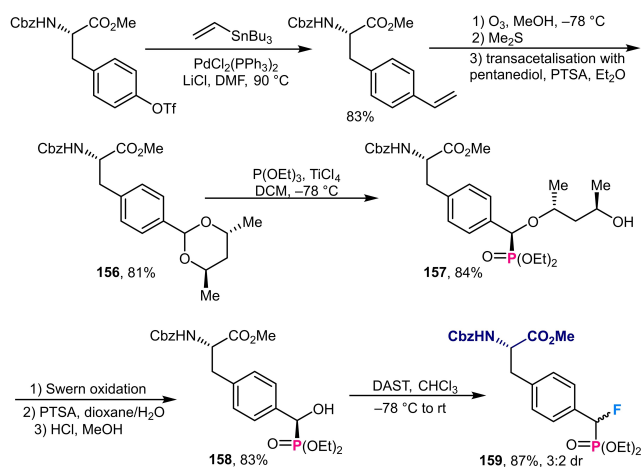
Scheme 58. Asymmetric transformation of tyrosine into 4-phosphonofluoromethyl-phenylalanine.
