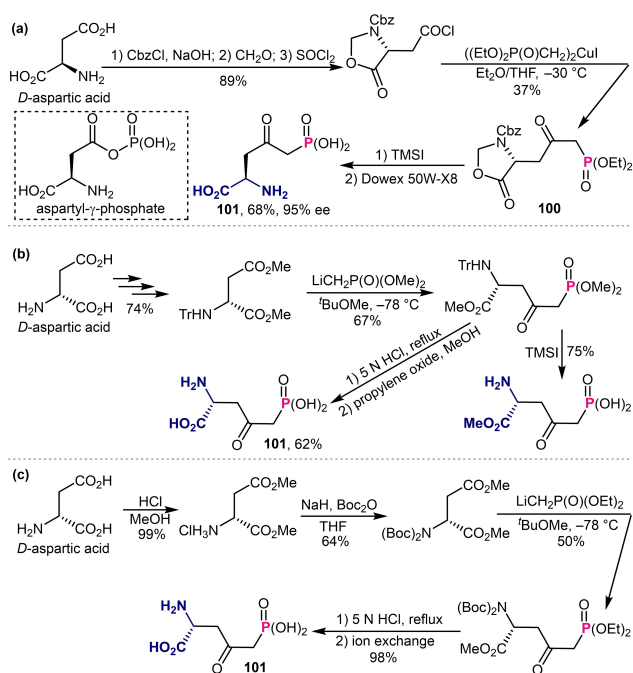
Scheme 35. Asymmetric transformation of D-Aspartic acid into ( R )- \gamma -keto- \delta -phosphonate \alpha -amino acid 101 .
