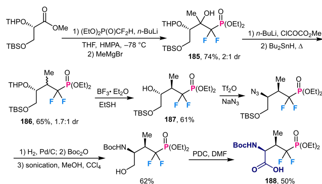
Scheme 69. Asymmetric transformation of methyl L-glycerate into N -Boc-protected CF 2 -pThr.
