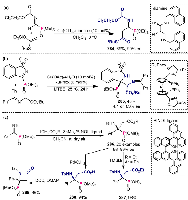
Scheme 97. Catalytic asymmetric construction of chiral \beta -phosphono- \beta -amino acid derivatives from iminophosphonates.
