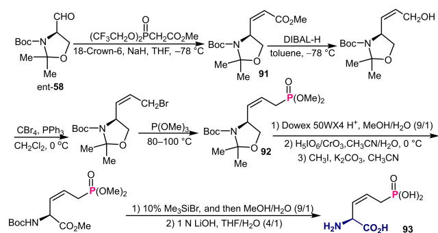
Scheme 32. Asymmetric synthesis of the ( Z )-2-amino-5-phosphono-3-enoic acid.
