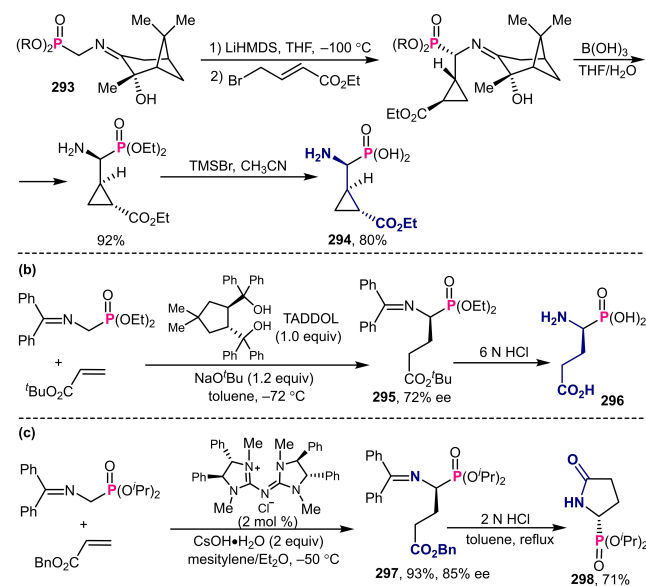
Scheme 99. Asymmetric construction of chiral \gamma -phosphono- \gamma -amino acid derivatives from iminophosphoglycinate derivatives.
