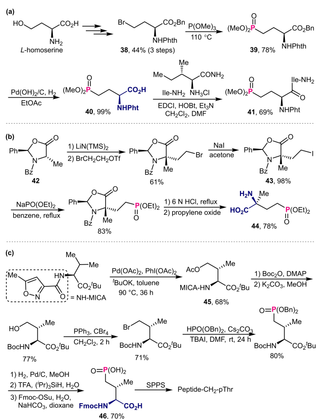
Scheme 14. The Michaelis–Becker reaction for the asymmetric synthesis of \gamma -phosphono- \alpha -amino acids.
