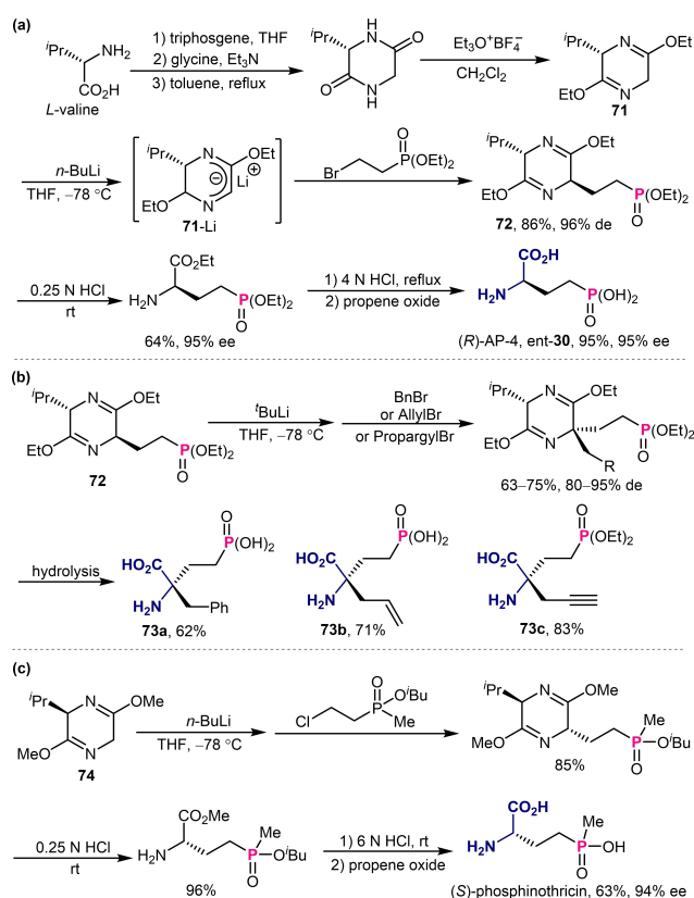
Scheme 23. Asymmetric alkylation of Schöllkopf bis-lactim ethers for the construction of \gamma -phosphono- \alpha -amino acid derivatives.
