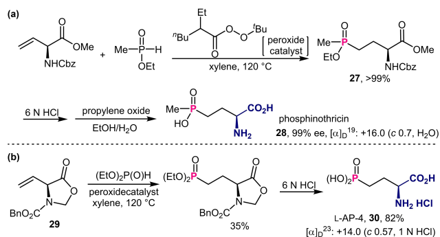
Scheme 11. Asymmetric transformation of vinylglycines into \gamma -phosphono- \alpha -amino acid derivatives.
