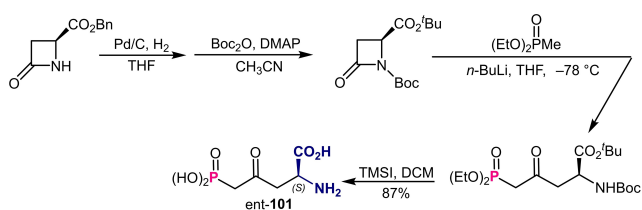
Scheme 36. Asymmetric transformation of chiral lactam into ( S )- \gamma -keto- \delta -phosphonate \alpha -amino acid.
