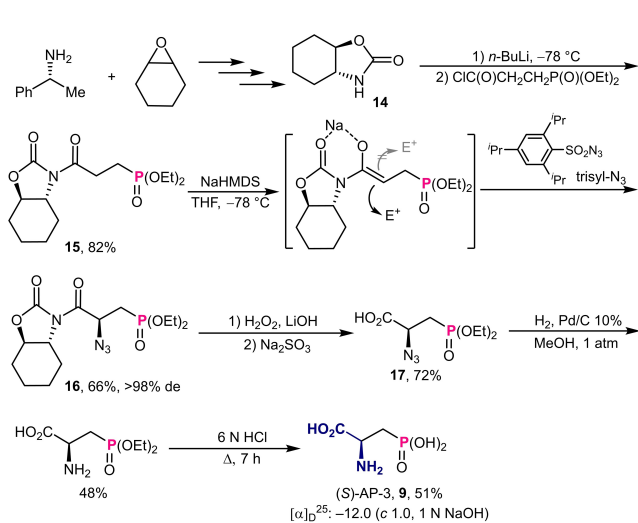
Scheme 6. Asymmetric azidation of N -acylated oxazolidinone for the synthesis of ( S )-AP-3.
