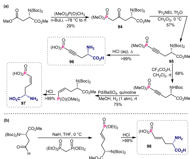
Scheme 33. Asymmetric synthesis of chiral acetylenic and Z/E -olefinic analogues of AP-5.
