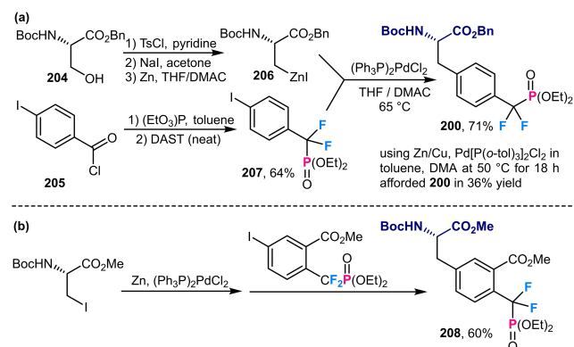
Scheme 75. Pd-catalyzed coupling of L-serine-derived zinc reagents with aryl iodide for the synthesis of F 2 Pmps.
