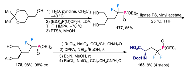
Scheme 66. Enzymatic desymmetrization for the asymmetric synthesis of the CF 2 -pSer mimic.
