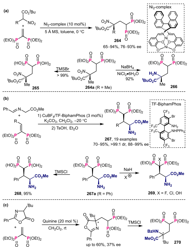
Scheme 91. Catalytic enantioselective syntheses of chiral bisphosphono- \alpha -amino acid derivatives.
