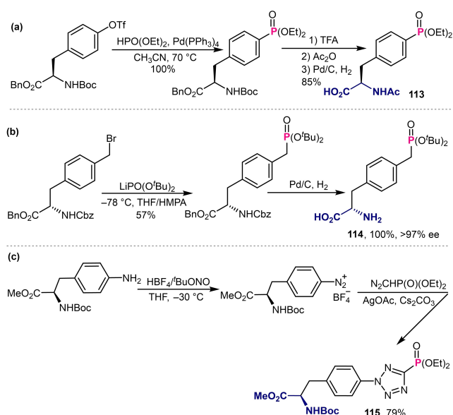
Scheme 42. Direct functionalization on the backbones of tyrosine and phenylalanine derivatives.
