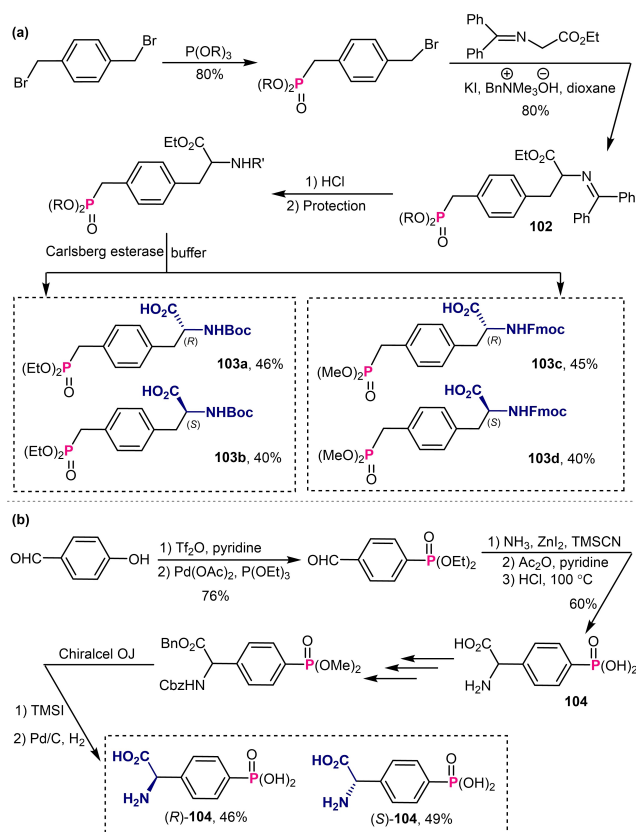
Scheme 37. Chiral resolutions for the preparation of enantiomers of Pmp and PPG.
