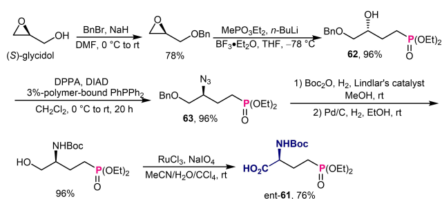
Scheme 19. Mitsunobu reaction for the asymmetric synthesis of \gamma -phosphono- \alpha -amino acid.
