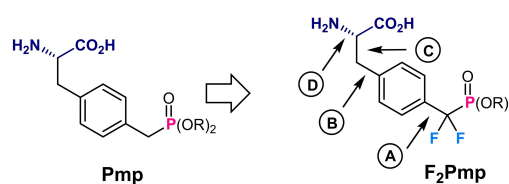
Figure 4. Structures of (phosphonomethyl)phenylalanine (Pmp) and (phosphonodifluoromethyl)phenylalanine ( \text{F}_2 Pmp).
