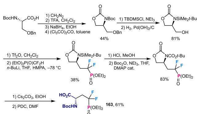
Scheme 60. Asymmetric transformation of L-serine into \beta -difluorophosphonomethyl- \alpha -amino acid.
