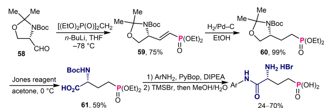
Scheme 18. Asymmetric transformation of Garner's aldehyde into \gamma -phosphono- \alpha -amino acid derivatives.
