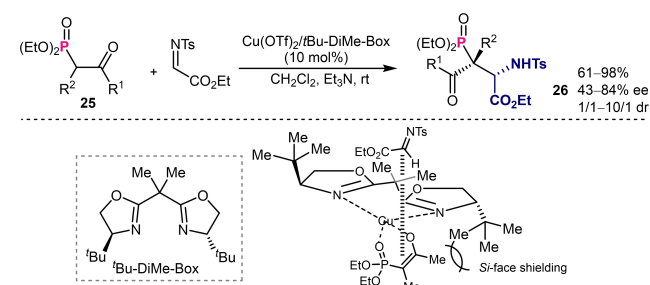
Scheme 10. Cu-catalyzed asymmetric synthesis of \beta -phosphono- \alpha -amino acid derivatives.
