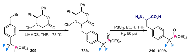
Scheme 76. Chiral Williams lactone-induced asymmetric synthesis of L-F 2 Pmp.
