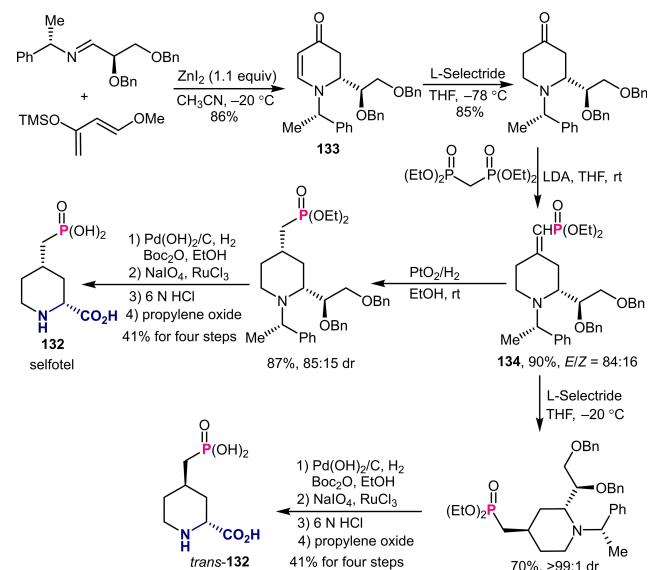
Scheme 49. Asymmetric stereodivergent synthesis of selfotel.
