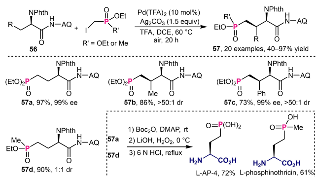
Scheme 17. Pd-catalyzed C(sp^3) -H alkylation for the asymmetric synthesis of \gamma -phosphono- \alpha -amino acid derivatives.
