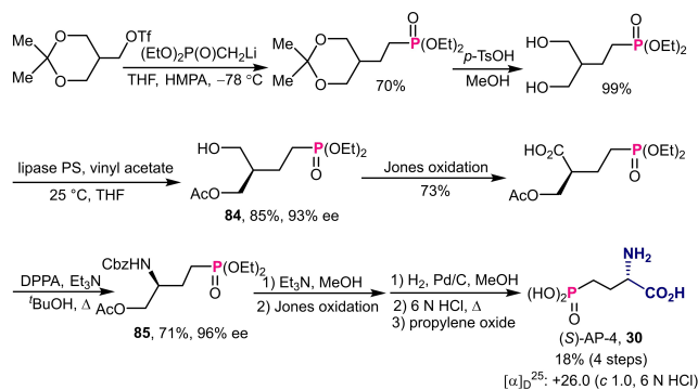
Scheme 28. Lipase-catalyzed enantioselective synthesis of ( S )-AP-4.
