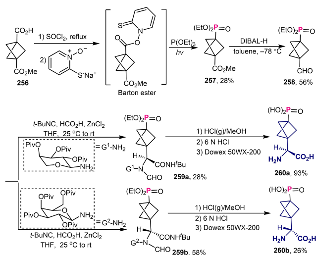
Scheme 89. Asymmetric synthesis of chiral phosphonobicyclo[1.1.1]pentyl amino acid derivatives.
