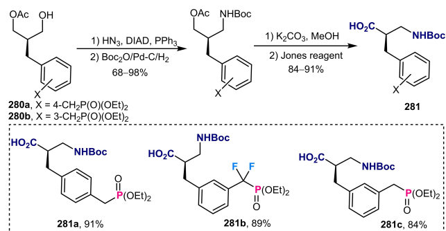
Scheme 95. Asymmetric transformation of chiral substrates into enantiomerically pure phosphonophenyl- \beta -amino acids.
