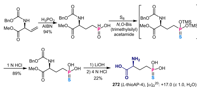
Scheme 93. Asymmetric transformation of chiral substrate into 2-amino-4-thiophosphonobutyric acid L-thioAP-4.
