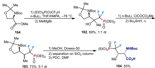
Scheme 68. Asymmetric transformation of chiral Garner's ester into difluorophosphonomethyl pThr derivative.
