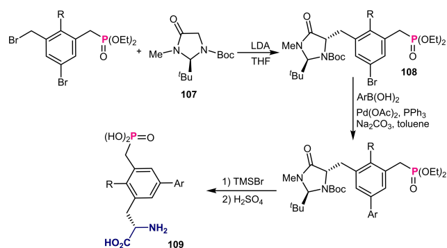
Scheme 39. Chiral imidazolidinone-induced asymmetric synthesis of Pmps.
