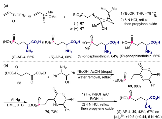
Scheme 22. Asymmetric transformation of chiral Schiff bases into AP-4 and phosphinothricin.
