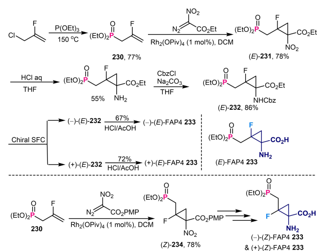
Scheme 83. Diastereoselective synthesis of 1-amino-2-fluoro-2-(phosphonomethyl)cyclopropane-1-carboxylic acids.
