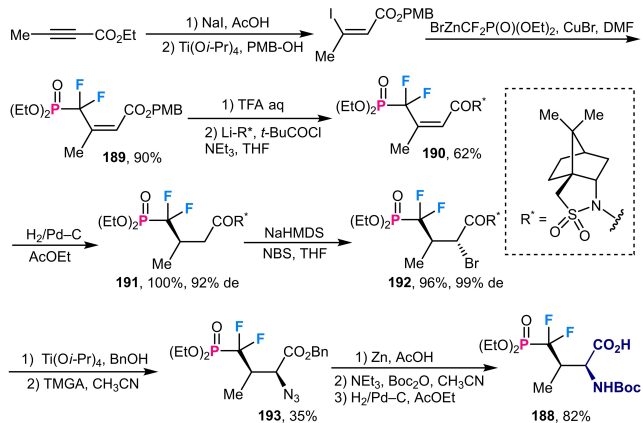
Scheme 70. Chiral auxiliary-induced asymmetric synthesis of N -Boc-protected \text{CF}_2 -pThr.
