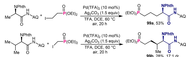
Scheme 34. Pd-catalyzed asymmetric synthesis of \delta -phosphono amino acid derivatives.
