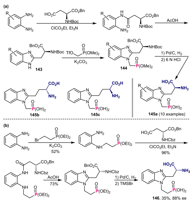
Scheme 53. Asymmetric synthesis of chiral benzimidazole-based phosphono- \alpha -amino acids.
