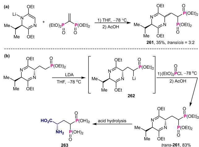
Scheme 90. Chiral auxiliary-induced diastereoselective synthesis of enantiopure bisphosphono- \alpha -amino acids.
