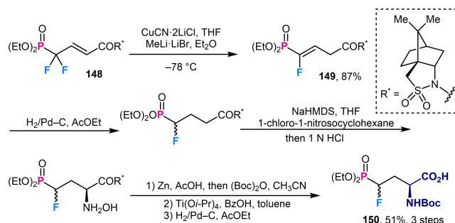
Scheme 55. Oppolzer's chiral sultam-induced asymmetric synthesis of monofluorophosphonomethyl-( S )-serine.
