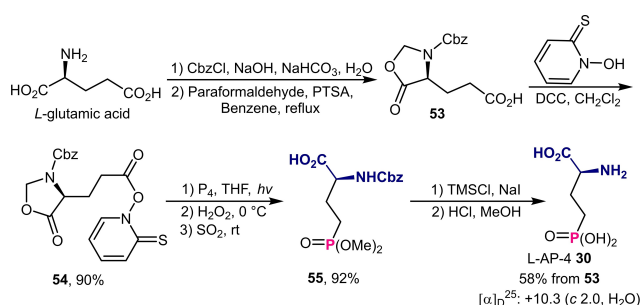
Scheme 16. Asymmetric transformation of L-glutamic acid to L-AP-4.
