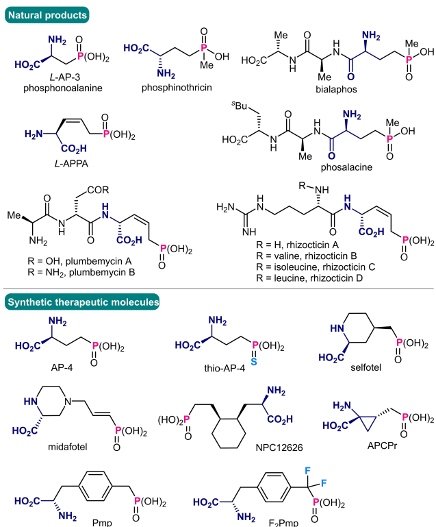
Figure 1. Naturally-occurring and representative man-made bioactive chiral amino carboxylic-phosphonic acid derivatives.
