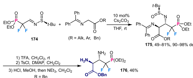
Scheme 65. Chiral auxiliary-induced asymmetric construction of a \beta -amino- \beta -difluorophosphonomethyl- \alpha -amino acid.
