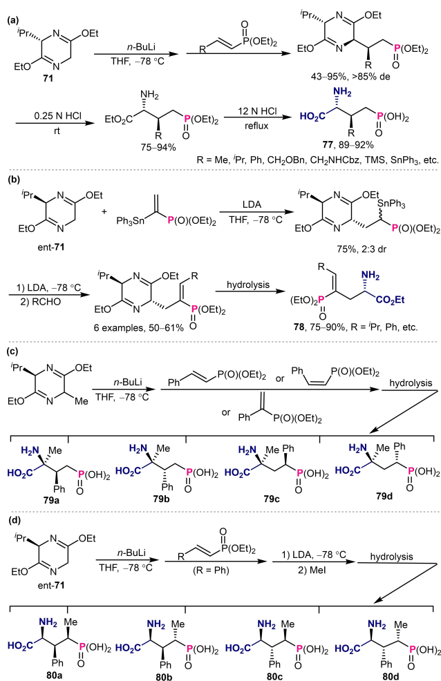
Scheme 25. Asymmetric synthesis of substituted AP-4 analogues.
