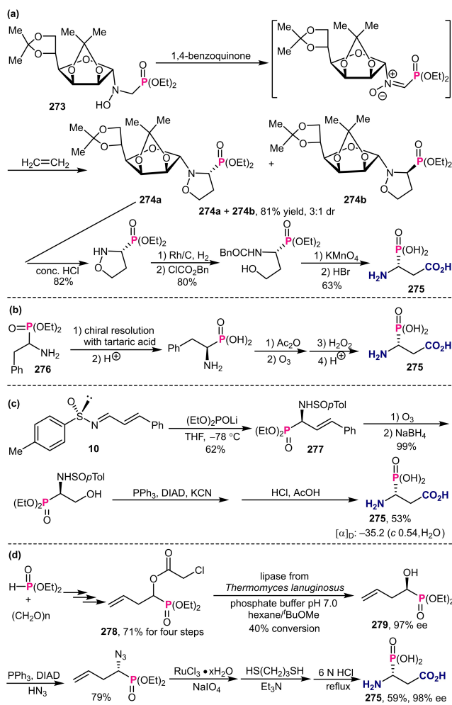
Scheme 94. Asymmetric construction of chiral \beta -phosphono- \beta -amino acid 275 .
