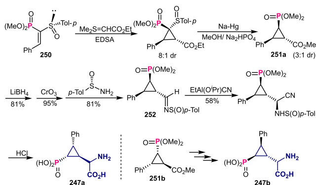
Scheme 87. Chiral sulfinyl-induced asymmetric construction of chiral phosphono-phenylcyclopropyl glycines.
