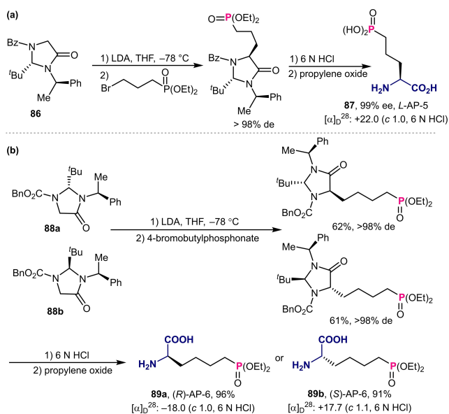
Scheme 29. Asymmetric transformation of chiral imidazolidinones into \delta - and \epsilon -phosphono- \alpha -amino acid derivatives.
