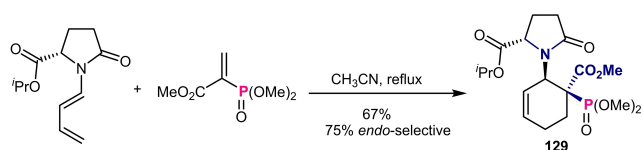
Scheme 47. Asymmetric [4 + 2] cycloaddition for the synthesis of chiral phosphonated 2-aminocyclohex-3-ene-1-carboxylate.
