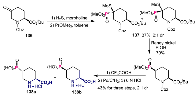
Scheme 51. Chiral substrate-induced asymmetric synthesis of 5-phosphonate pipercolic acids.
