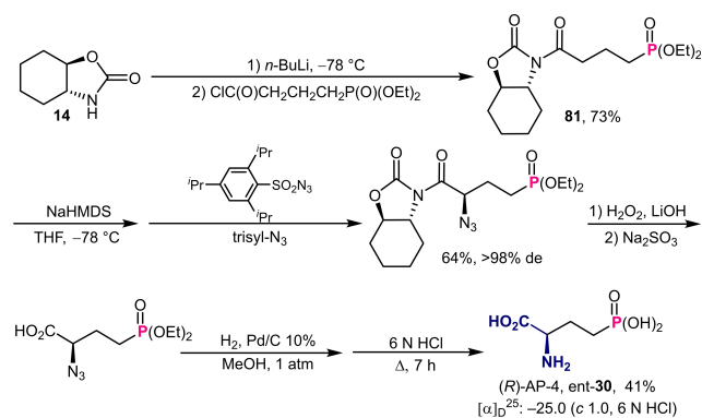
Scheme 26. Asymmetric transformation of chiral oxazolidinone into ( R )-AP-4.
