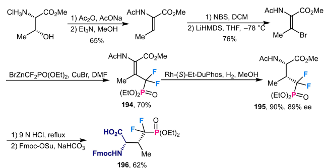
Scheme 71. Catalytic asymmetric hydrogenation for the synthesis of N -Fmoc-protected \text{CF}_2 -pThr.
