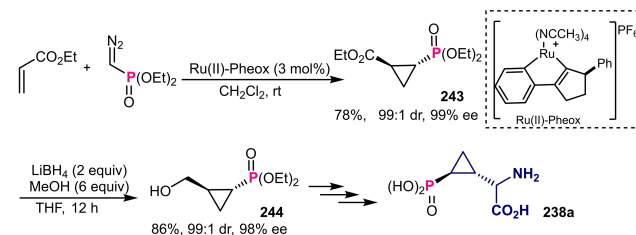
Scheme 85. Catalytic asymmetric synthesis of chiral phosphonocyclopropyl glycine precursor.
