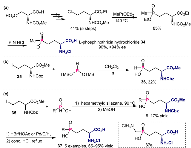
Scheme 13. The Michaelis–Arbuzov reaction for the asymmetric construction of \gamma -phosphono- \alpha -amino acids.
