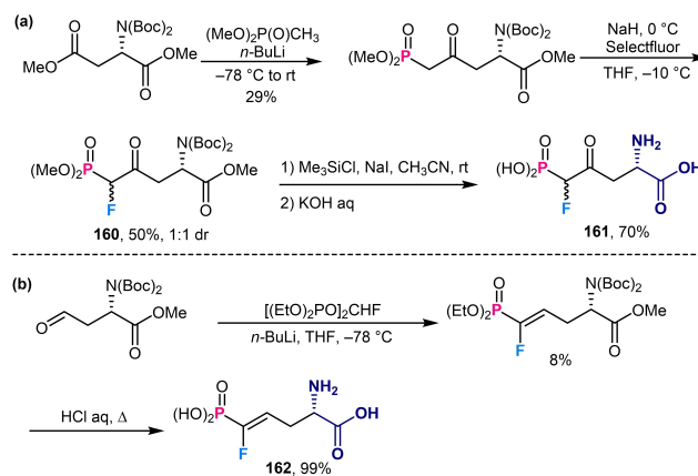
Scheme 59. Asymmetric transformation of chiral substrates into monofluorophosphonomethyl aspartic acid derivatives.
