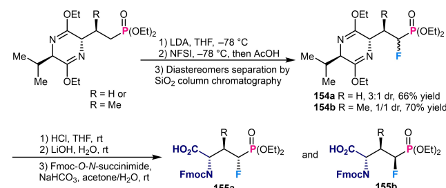
Scheme 57. Chiral Schöllkopf bis-lactim ether-induced asymmetric construction of monofluorophosphono- \alpha -amino acids.
