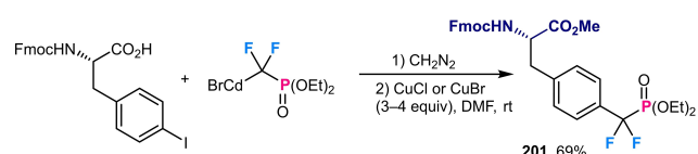
Scheme 73. Cu-mediated cross-coupling of L-4-iodophenylalanine and (EtO) 2 POCF 2 CdBr for the synthesis of F 2 Pmp.
