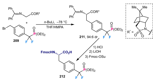
Scheme 77. Chiral camphorsultam glycine imine-induced asymmetric synthesis of N -Fmoc-protected L-F 2 Pmp.
