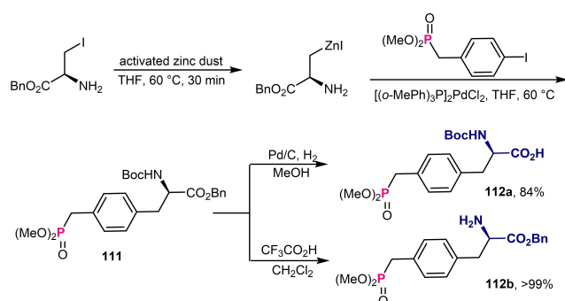
Scheme 41. Asymmetric transformation of iodo-derived serine into chiral Pmps.
