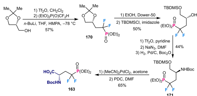
Scheme 63. Asymmetric transformation of ( R )-solketal into the CF 2 -pSer mimic.
