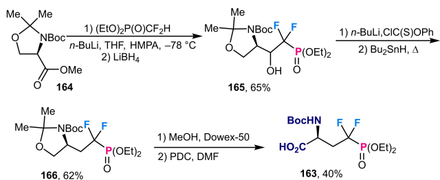
Scheme 61. Asymmetric transformation of D-serine-derived Garner's ester into \beta -difluorophosphonomethyl- \alpha -amino acid.
