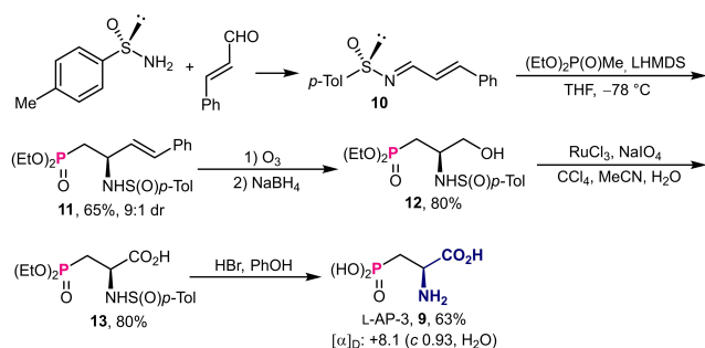
Scheme 5. Asymmetric 1,2-addition of (\text{EtO})_2\text{P}(\text{O})\text{Me} to enantiopure sulfinimine for the synthesis of 3-phosphono-alanine.
