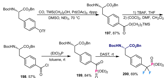
Scheme 72. Asymmetric transformation of natural L-tyrosine into the F 2 Pmp derivative.
