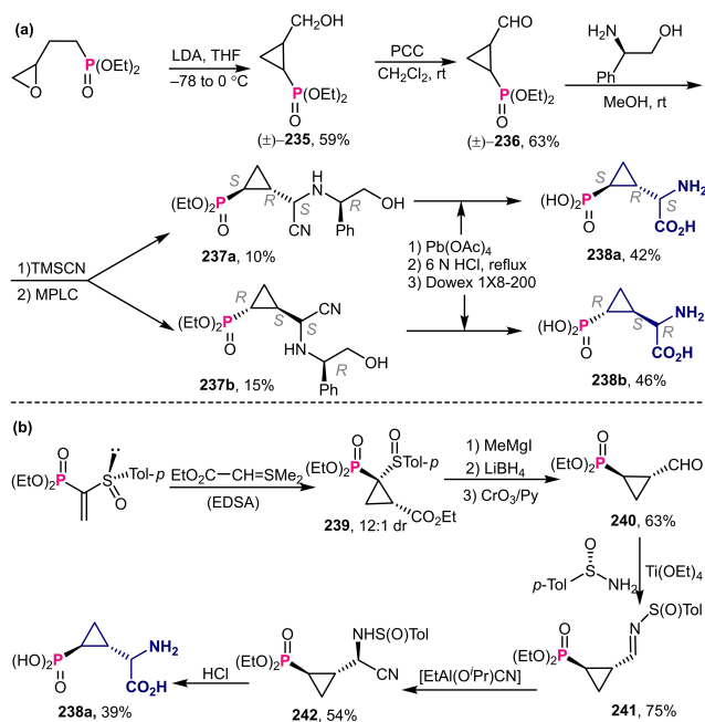
Scheme 84. Diastereoselective synthesis of phosphono-cyclopropyl glycine (PCG) derivatives.
