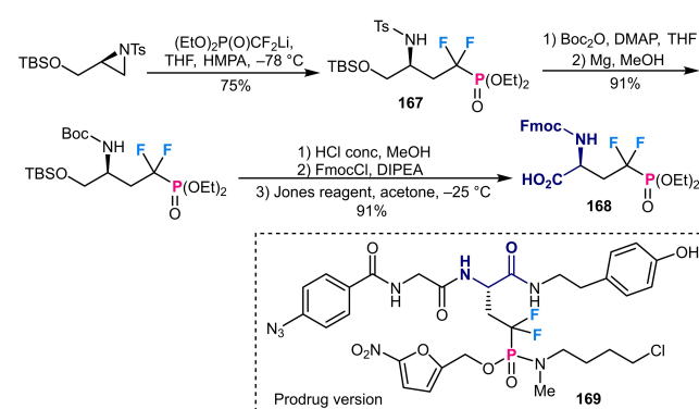
Scheme 62. Asymmetric transformation of enantiomerically pure aziridine into chiral phosphoserine.
