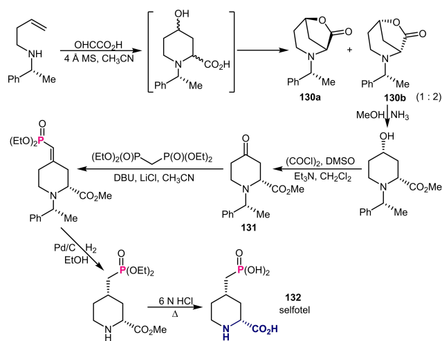
Scheme 48. Chiral auxiliary-induced asymmetric synthesis of selfotel.
