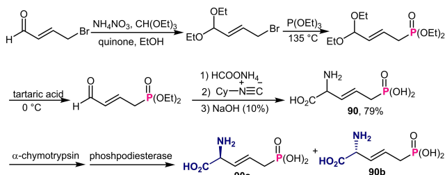
Scheme 31. Enzymatic asymmetric construction of unsaturated \delta -phosphono- \alpha -amino acids.
