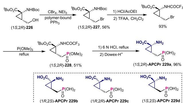
Scheme 82. Asymmetric transformation of chiral cyclopropyl \alpha -amino acids into enantiopure APCPrs.
