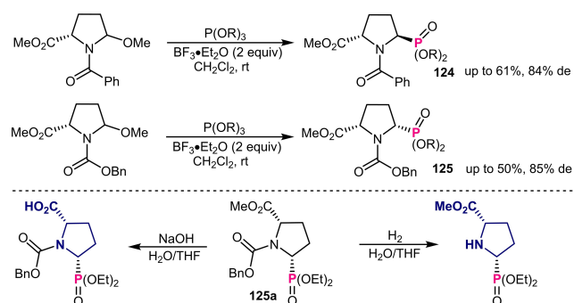
Scheme 45. Asymmetric synthesis of chiral 5-phosphonate proline derivatives.
