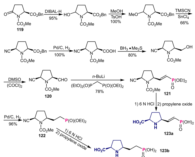
Scheme 44. Asymmetric transformation of ( S )-pyroglutamate into chiral proline-based phosphonic acids.
