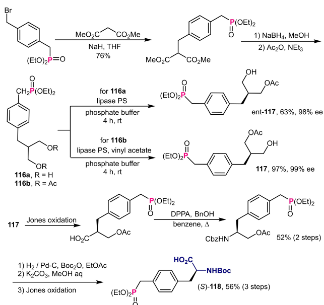
Scheme 43. Enzymatic desymmetrization for enantioselective synthesis of Pmp.
