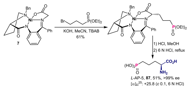
Scheme 30. Asymmetric transformation of chiral Schiff base Ni-complex into \delta -phosphono- \alpha -amino acid L-AP-5.
