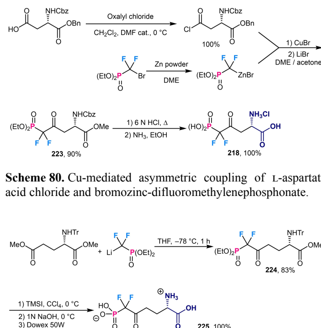
Scheme 81. Asymmetric transformation of N -trityl-L-glutamic acid ester into difluorophosphonomethyl glutamate analogue.
