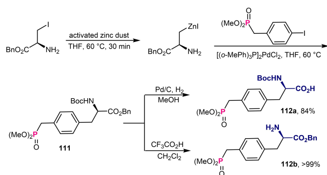
Scheme 41. Asymmetric transformation of iodo-derived serine into chiral Pmps.
