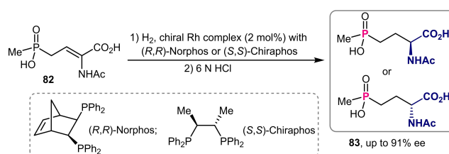
Scheme 27. Rh-catalyzed asymmetric synthesis of both enantiomers of phosphinothricin.
