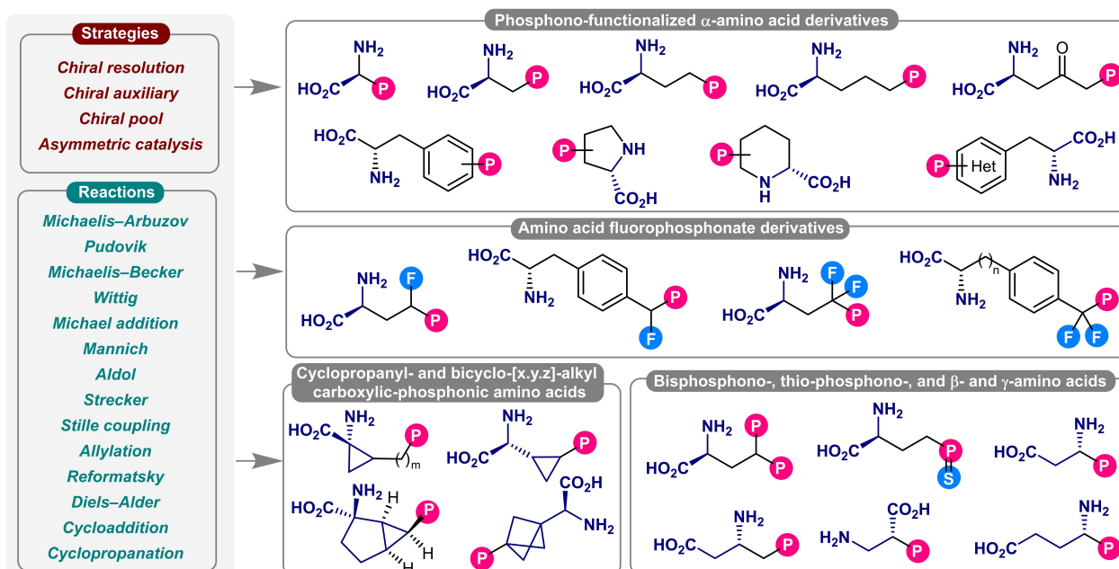
Figure 2. Representative chiral amino carboxylic-phosphonic acid derivatives, key strategies, and reactions.
