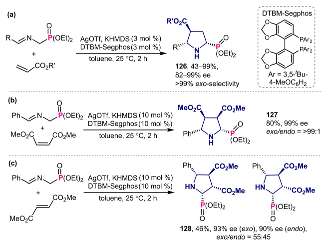
Scheme 46. Catalytic asymmetric cycloaddition reactions for the synthesis of chiral phosphonic proline-analogues.
