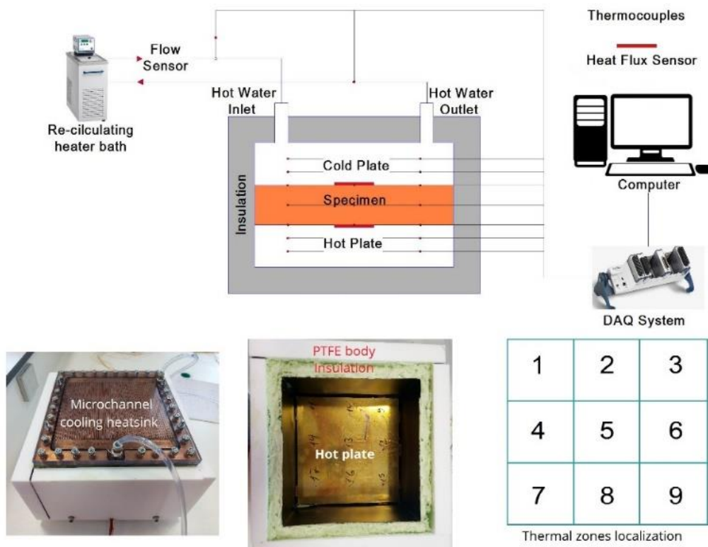
Fig. 2. Components of the test bench
