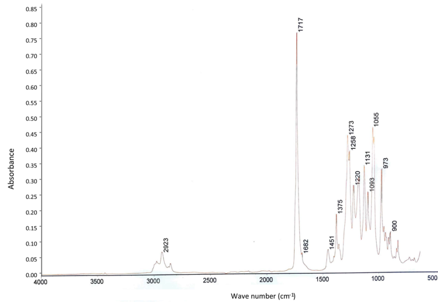
Figure 3. FTIR spectrum of PHAs produced by HW T5.17 T strain ( Acidisoma cellulolytica ) grown on TSB depleted in nitrogen and supplemented with glucose as sole carbon source (a similar spectrum was obtained with strain HW T2.11 T ).
