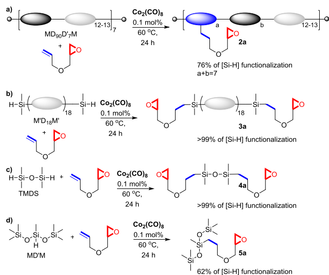
Scheme 3. Determining the role of intramolecular [Si-H] concentration in (poly)silane towards the cross-linking of PMHS with C=O and epoxide groups. a Same reaction conditions as in Scheme 2. Reaction scale for a), b) and d): silane (0.55 mmol [Si-H], 1 equiv.), AGE (0.55 mmol 1 equiv.); for c) silane (0.55 mmol, 0.5 equiv.), AGE (1.10 mmol 1 equiv.).
