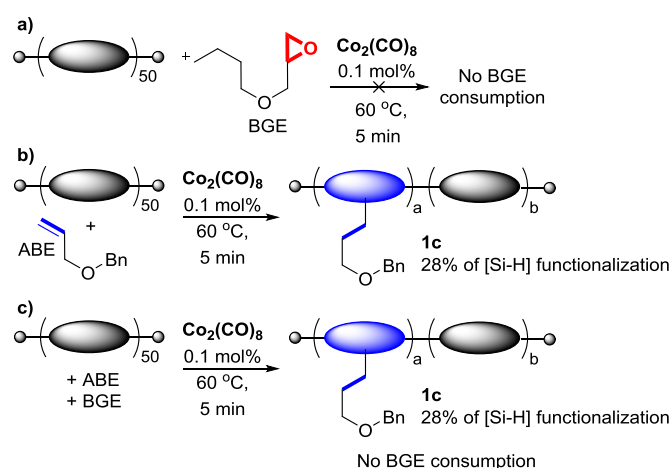
Scheme 4. Determining the role of allyl and epoxide groups in the PMHS cross-linking with AGE. a Same reaction conditions as in Scheme 2. Reaction scale for a)-b): PMHS (2.34 mmol [Si-H], 1 equiv.) and BGE or ABE (2.34 mol, 1 eq.). c) PMHS (2.34 mmol [Si-H], 1 equiv.), BGE (2.34 mol, 1 equiv.) and ABE (2.34 mol, 1 equiv.). Bn-benzyl.
