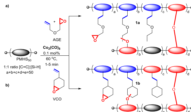
Scheme 2. Cross-linking of PMHS with AGE and VCO. Reaction conditions: alkene (3.75 mmol, 1.0 eq), PMHS (3.75 mmol, 1.0 eq), Co_2(CO)_8 (0.1 mol% compared to [Si-H]) in toluene. The samples were further post-cured at 60 °C until the end of 24 h of reaction time.
