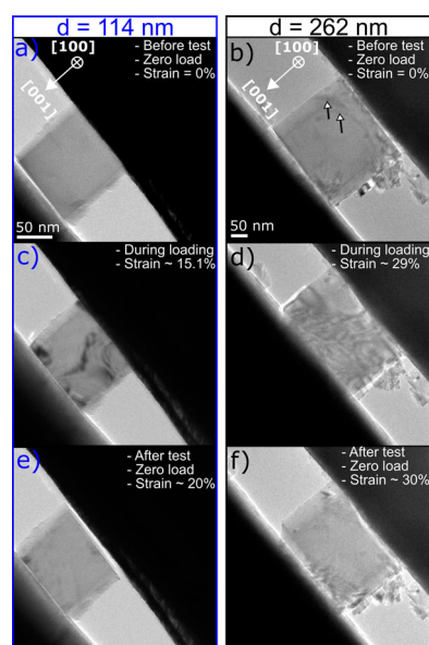
Figure 1. BF TEM images of MgO nanocubes (near [100] zone axis) extracted from compression tests along the [001] direction. (a,c,e) nanocube of size 114 nm before load, at \sim 15.1\% and \sim 20\% strain. (b,d,f) nanocube of size 262 nm before load, at \sim 29\% and \sim 30\% strain. Two dislocations are indicated by black arrows.
