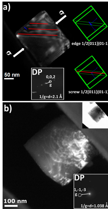
Figure 2. TEM images of nanocubes at different stages of in situ compression tests. (a) WBDF TEM image using the diffraction vector (002) of a 195 nm nanocube at yield stress. Crystallographic models are shown in the inset. (b) WBDF image of a 355 nm sized cube at zero load after 22% true strain (diffraction vector used g = [1\bar{1}\bar{3}] ).
