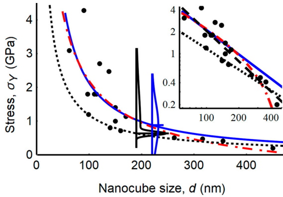
Figure 4. Dependence of the yield stress on the nanocube size. The experimental points ( \bullet ) are fitted to \sigma = ad^{-x} and \sigma = ad^{-x} + \sigma_0 using LS fitting on linear axes (blue lines and chain-dotted red lines, respectively). A LS fitting of a straight line on log-log axes is shown in the inset (dashed black line). The dotted black lines are the result of the outcome of the Maximum Likelihood (ML) fit calculated for \sigma = ad^{-x} with three parameters defining an asymmetric probability distribution functions of the residuals. The two graphs plotted above the 200 nm tickmark show the LS Gaussian pdf (blue) and the ML pdf (black) for the residuals, centred on the respective curves of best fit.
