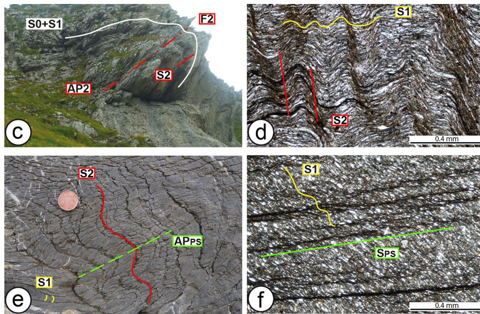
Figure 3. Outcrop- and micro-scale structural features in the Marguareis Unit. (a) F1 fold with AP1 axial plane and S1–S2 overprint; (b) S1 foliation; (c) F2 fold which folds the S0–S1 surface. AP2 axial plane and S2 foliation are indicated; (d) S1–S2 interference pattern at the microscale; (e) S1 and S2 foliations folded by AP PS axial plane; (f) S PS foliation which folds the S1. SO: bedding.
