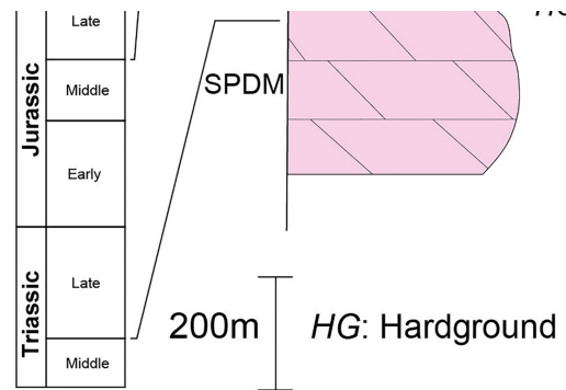
Figure 2. Stratigraphic log of Marguareis Unit (modified and re-draw from Brizio et al., 1983).
