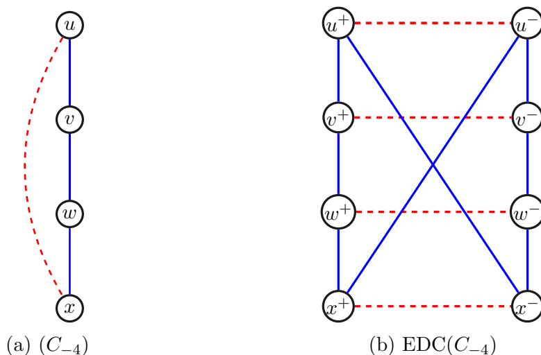
Figure 1: Signed graphs C_{-4} and \text{EDC}(C_{-4}) . Dashed (red) edges are negative.
