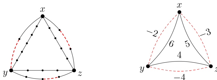
Figure 2: T_g(p, q, r) with g = 8 , p = 6 , q = -4 , and r = -3 . Dashed (red) edges are negative.
