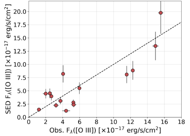
Figure 7. Comparison of [O\ III] + H\beta line fluxes measured from the best-fitting SED and K -band excess and the observed line fluxes from NIR spectra. From the limited number of galaxies in our sample that have observed line fluxes from Cullen et al. (2021), we can conclude that our method of estimating line fluxes from K -band excess works reasonably well.
