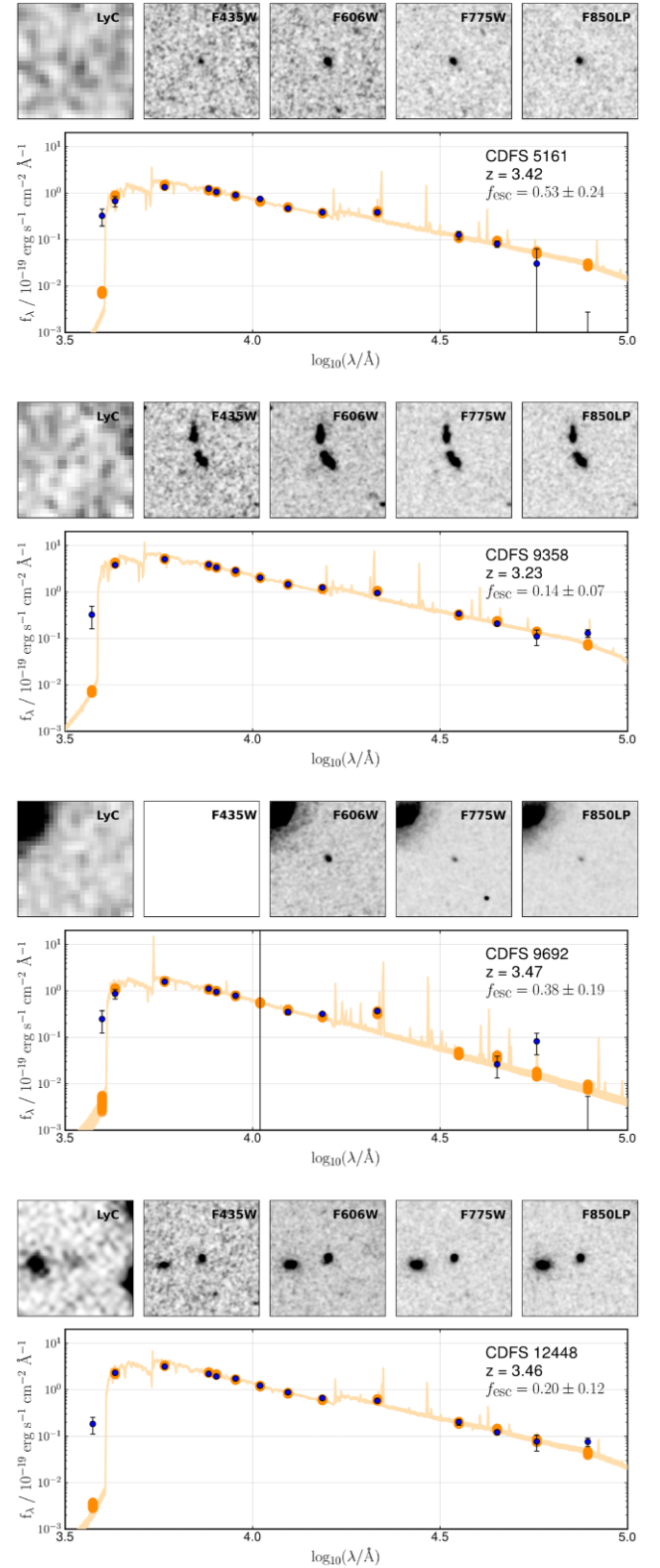
Figure A1. LyC and HST photometry (top), and best-fitting SED (orange) with observed (blue points) and SED derived (orange ovals) for candidate LyC leaking galaxies. We show the observed and SED predicted flux at LyC wavelengths only for demonstration purposes – the SED derived LyC fluxes were not used to infer f_{\text{esc}} and the observed LyC fluxes were not used during SED fitting to obtain galaxy physical properties.
