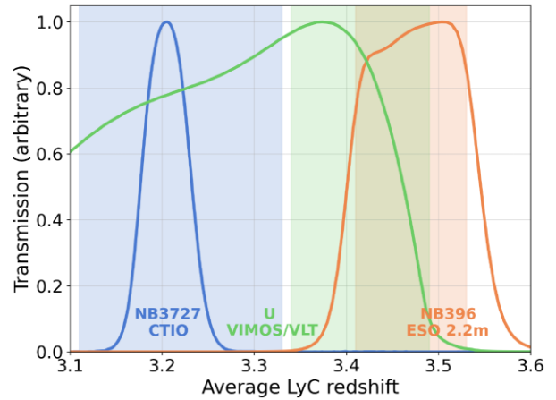
Figure 1. Filter transmission profiles of the NB3727, NB396, and the U-band filters used to target LyC emission in this study. The x-axis shows the redshift at the rest-frame wavelength of 886 Å, which is the mid-point wavelength of the LyC emission sampled between 860 < \lambda < 912 \text{ Å} in this study (shaded regions for each filter). More details about the filter properties and LyC redshift ranges covered are given in Section 2.1.
