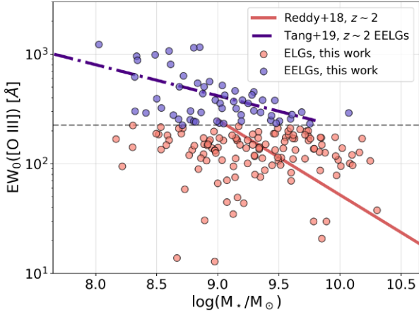
Figure 6. Distribution of EW_0([O\ III]) and galaxy stellar mass derived for our sample of galaxies using SED fitting. Shown for comparison are the best-fitting relations derived between the two quantities for relatively massive star-forming galaxies at z \sim 2 by Reddy et al. (2018) (red solid line) from the MOSDEF survey and extreme emission line galaxies (EELGs) at z \sim 2 by Tang et al. (2019) (blue dot-dashed line), where the black dashed line marks EW_0([O\ III]) > 225\ \text{\AA} , used by Tang et al. (2019) to classify galaxies as EELGs. The normalization of the best-fitting relations have not been altered. Galaxies from our sample that would be considered as normal emission line galaxies (ELGs) are shown as red points, and those considered as EELGs are shown using blue points. The distribution of our SED derived measurements (and the scatter) are broadly consistent with spectroscopic measurements at lower redshifts.
