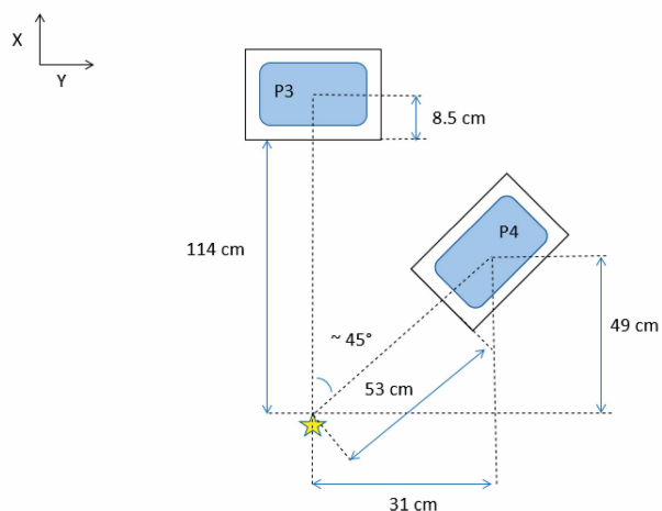
FIG. 2. Setup 2 with two phantoms, one homogenously exposed, P3, and one laterally exposed, P4. The figure includes the dimensions used for Monte Carlo simulation of the exposure geometry. The star indicates the position of the ^{192}\text{Ir} source.
