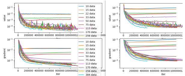
Fig. 7: Comparison of sample size needed to achieve sufficient accuracy with classical and Sobolev regression (left) with Sobolev loss (right) without Sobolev loss. The Sobolev loss is less prone to be stuck in a local minimum when smaller dataset are provided when approximating the value (top). The derivative of the value is always better approximated with Sobolev loss (bottom).
