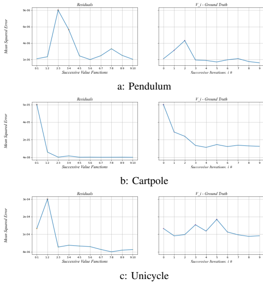
Fig. 3: Bellman residuals i.e difference between the value at two successive iterations (left) and difference between value function at each iteration and ground truth (right)
