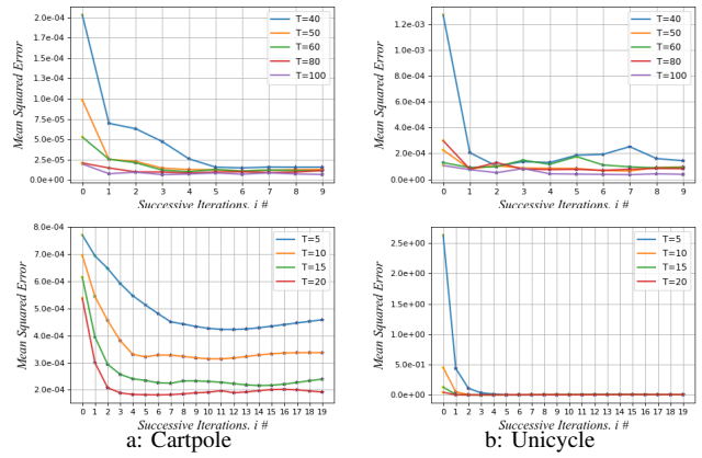
Fig. 5: Evolution of the difference between ground truth value function and different iterations, for high horizons (top) and small horizons (low).
