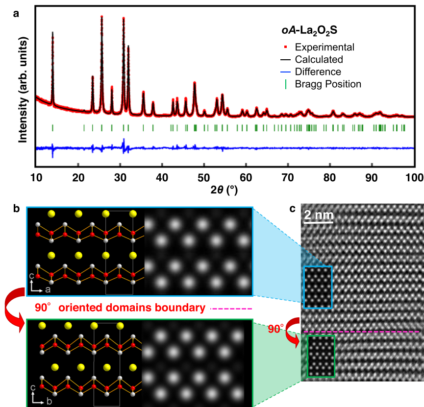
Fig. 2 Structure characterization of oA -La 2 O 2 S. a Experimental XRD pattern of oA -La 2 O 2 S obtained by the reaction of La 2 O 2 S 2 with Rb 0 metal at 350 °C. The Rietveld refinement was conducted using as input the structure predicted by USPEX. b Simulated HAADF-STEM images viewed along [010] and [100] directions obtained using the refined structure of oA -La 2 O 2 S. In the projected structure lanthanum, oxygen, and sulfur atoms are represented by white, red, and yellow balls, respectively. c The experimental HAADF-STEM image of oA -La 2 O 2 S superimposed by each of the simulated images. Only La atoms were observed as bright spheres (ADF signal is proportional to the n th power of the atomic number, with n -2).
