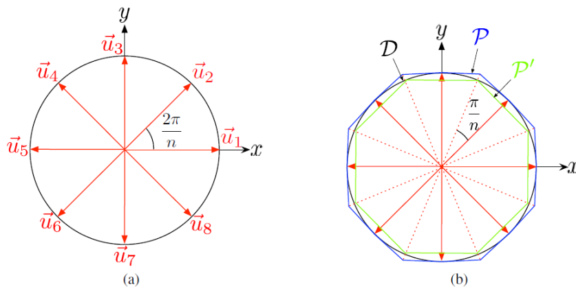
Figure 1: Linearization of the euclidean norm of \mathbb{R}^2 for 8 directions (Camino et al. [2021])
