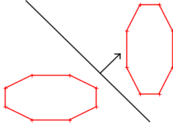
Figure 9: Linear separation of two ellipses outer approximations by the black line
