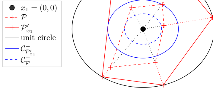
Figure 4: Inflation of \mathcal{P} by x_1 = (0, 0)
