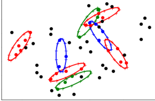
Figure 13: Example of a feasible solution with the ellipse model
