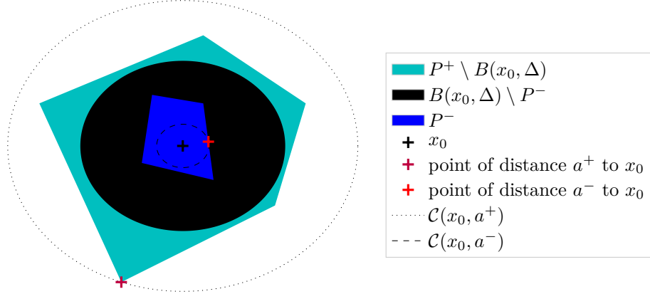
Figure 2: Illustration of Definition 1
