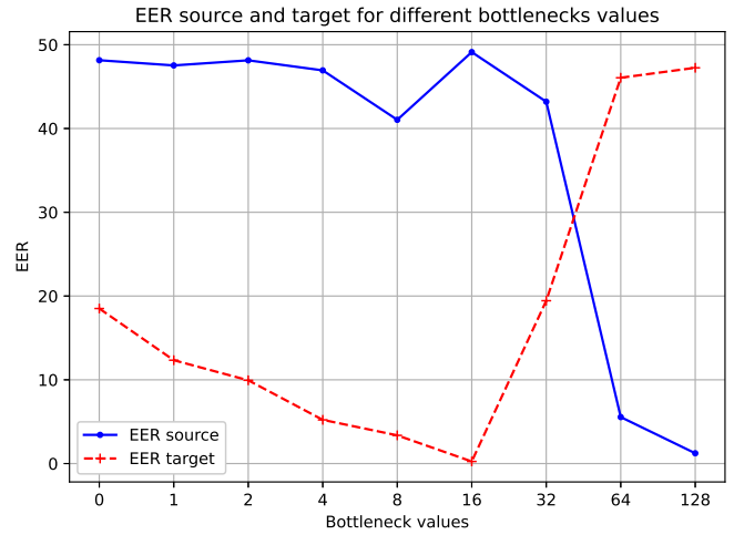
Fig. 3. Graph of the EER_{source} and EER_{target} for different bottlenecks values, computed on the \mathbf{E}_{VST_{Test}} set.
