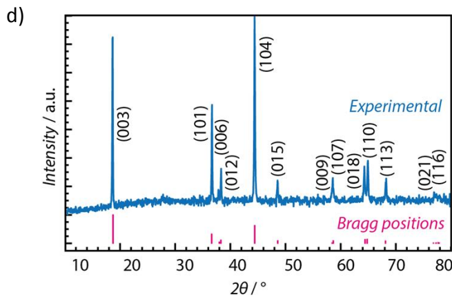
684 Fig. 1. a) Schematic description of the different sources of polarization at different size levels of samples. b) 685 SEM images of NMC532 clusters and particles. c) EDS spectrum analysis (0-8 keV) of NMC532. d) X-ray 686 diffraction patterns using a PANalytical XPert Pro diffractometer: Cu-K \alpha : \lambda=1.5408\text{\AA} and step size of 0.017^\circ.s^{-1} . 687 e) Schematic structure of NMC532.
