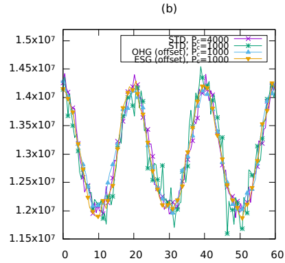
Figure 5. Non linear Landau damping: Density profile of the electron density (as a function of y ) at t = 6.3\omega_p^{-1} and x = \frac{L}{2} .
