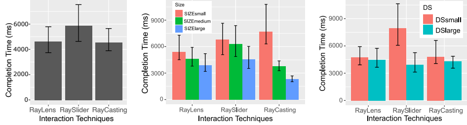
(a) Mean completion times. (b) Completion times according to the size of the target. (c) Completion times according to the density spacing.
