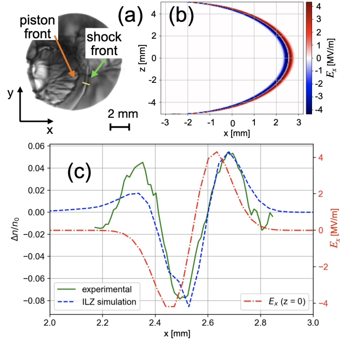
FIG. 4. Proton radiography obtained with the setup shown in Fig. 1, 5 ns after the laser pulse. (a) Raw dose collected on the RCF film corresponding to 19 MeV protons. (b) Hemispherical electric field E_x in the xz-plane, with a radius of R = 5.1 \text{ mm} , estimated from (a). (c) Lineout of the proton dose modulation along the yellow line indicated in (a). The green full curve is the modulation from the experimental results, and the dashed blue curve is that from the ILZ simulation, which is obtained by imposing a bipolar electric field with hemispherical shape shown in (b). The red dash-dotted curve represents the lineout of the field E_x in z = 0 .
