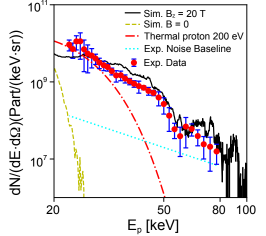
FIG. 7. Proton energy spectrum. The experimental data is shown with red dots and blue error bars; the 1D PIC simulation results are shown with black solid line for the case with B = 20 \text{ T} and yellow dashed line for B = 0 case; the analytical thermal proton spectrum is shown with red dash-dot line (200 eV); and the experimental noise baseline is shown in cyan dotted line. Note that the absolute scale in proton numbers (i.e., the number of protons per bin of energy, divided by the solid angle subtended by the entrance pinhole of the spectrometer) applies only to the experimental spectrum; the simulated spectra are adjusted to the experimental one.
