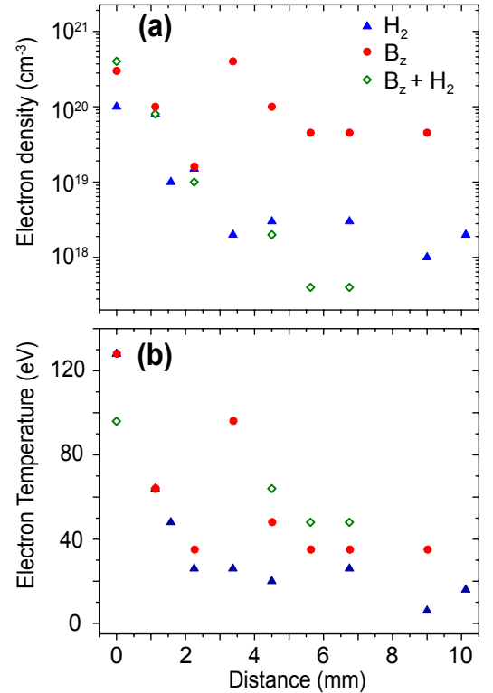
FIG. 3. FSSR evaluation of (a) electron density and (b) electron temperature of the laser-produced piston in three different configurations (see legend) along the expansion axis. The measurements are based on the analysis 50 of the relative intensities of the x-ray emission lines of He-like and H-like (see text) Fluorine ions in the expanding plasma in the range of 13\text{--}16 Å. The quasi-stationary 49 approach was applied for He-like series of spectral lines assuming a “frozen” ion charge state. The 0 point corresponds to the target surface. A spatial resolution of about 100\text{ }\mu\text{m} was achieved. The signal is time-integrated.
