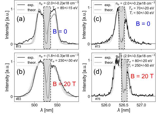
FIG. 6. Thomson scattering measurements, of the plasma density and temperatures, in the region downstream of the shock front, and for different cases. (a) measurement on the electron waves for B = 0 case (i.e. with only ambient gas), allowing to retrieve the local electron number density and electron temperature, as stated; (b) the same measurement for B = 20 T case (i.e. with external B-field and ambient gas). (c) measurement on the ion waves in the plasma for B = 0 case, allowing to retrieve the local electron and ion temperatures, as stated; (d) the same measurement for B = 20 T case. Solid lines are for experimental data profiles, while dashed lines are for theoretical spectra. The stated uncertainties in the retrieved plasma parameters represent the possible variation of the parameters of the theoretical fit (materialized by the thin dashed grey lines). Note that the deep central dip in the experimental spectra is related to a filter (a black aluminum stripe) which is positioned right before the entrance of the two streak cameras (recording respectively the light scattered off the electron and ion waves). This filter is used to block the very intense and unshifted laser wavelength (the Rayleigh-scattered light), which otherwise would saturate the cameras. Thus, no signal is recorded in this zone, which is materialized by the grey dashed box. The strong narrow peak at around 562.4 nm in panel (d) is caused by leakage of that strong light just at the edge of the filter. The position of the filter can change in the wavelength domain because the diagnostic can be realigned between shots.
