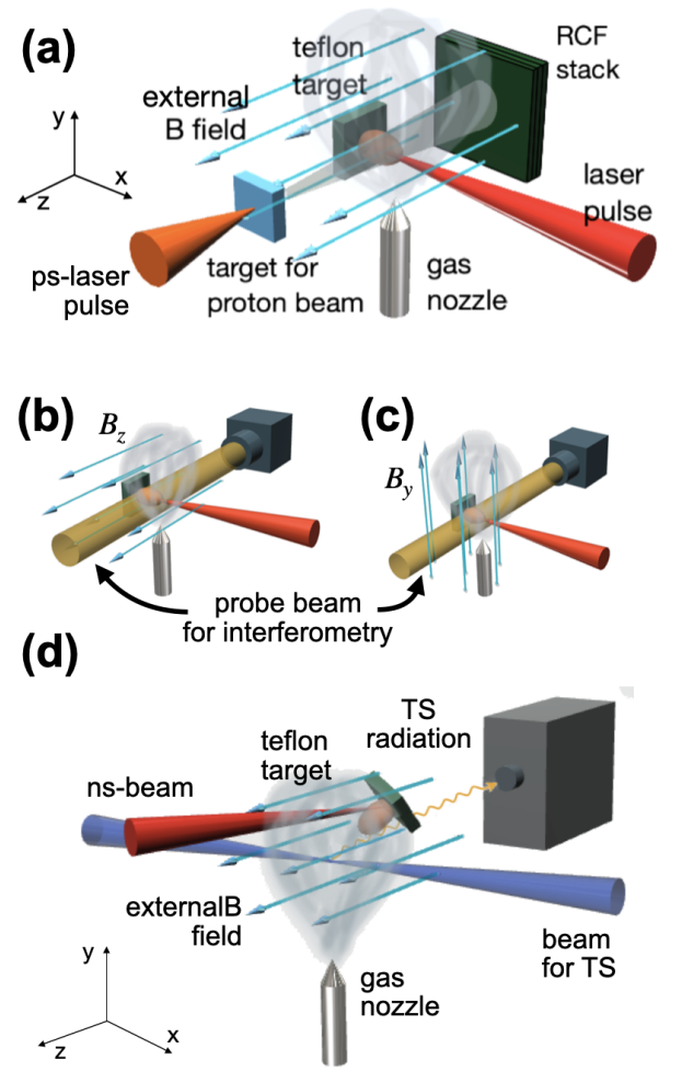
FIG. 1. Experimental setup and diagnostics used to characterize a magnetized shock. Proton radiography and interferometry diagnostics have been used alternatively along the axis perpendicular to the laser and to the plasma flow (i.e. the z-axis). (a) Proton radiography setup. (b-c) In the case of interferometry, we could rotate the coil in order to have two different magnetic field orientations with respect to the field of view of the probe beam. (d) Setup of the Thomson scattering (TS) diagnostic fielded at LULI2000.
